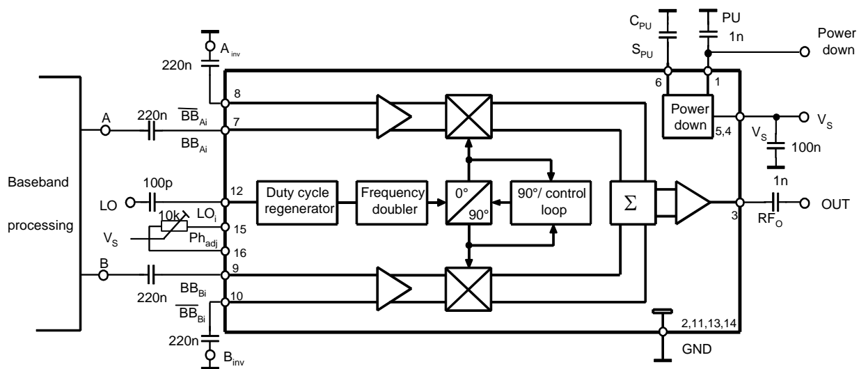
Figure 18. Application Circuit
