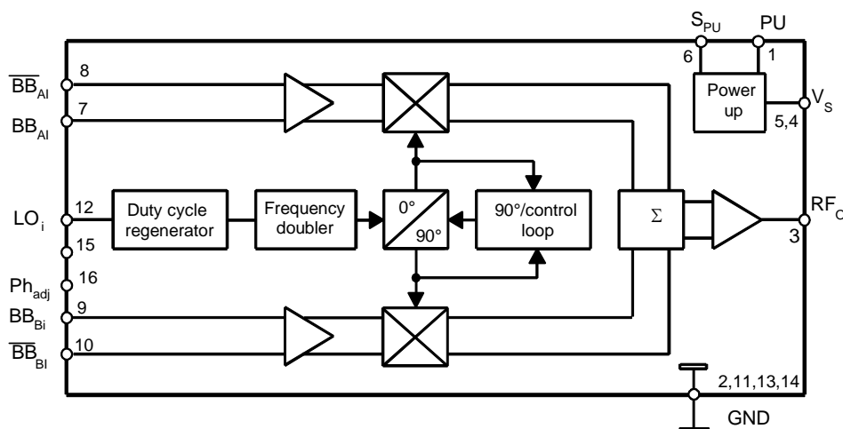
Figure 1. Block Diagram
