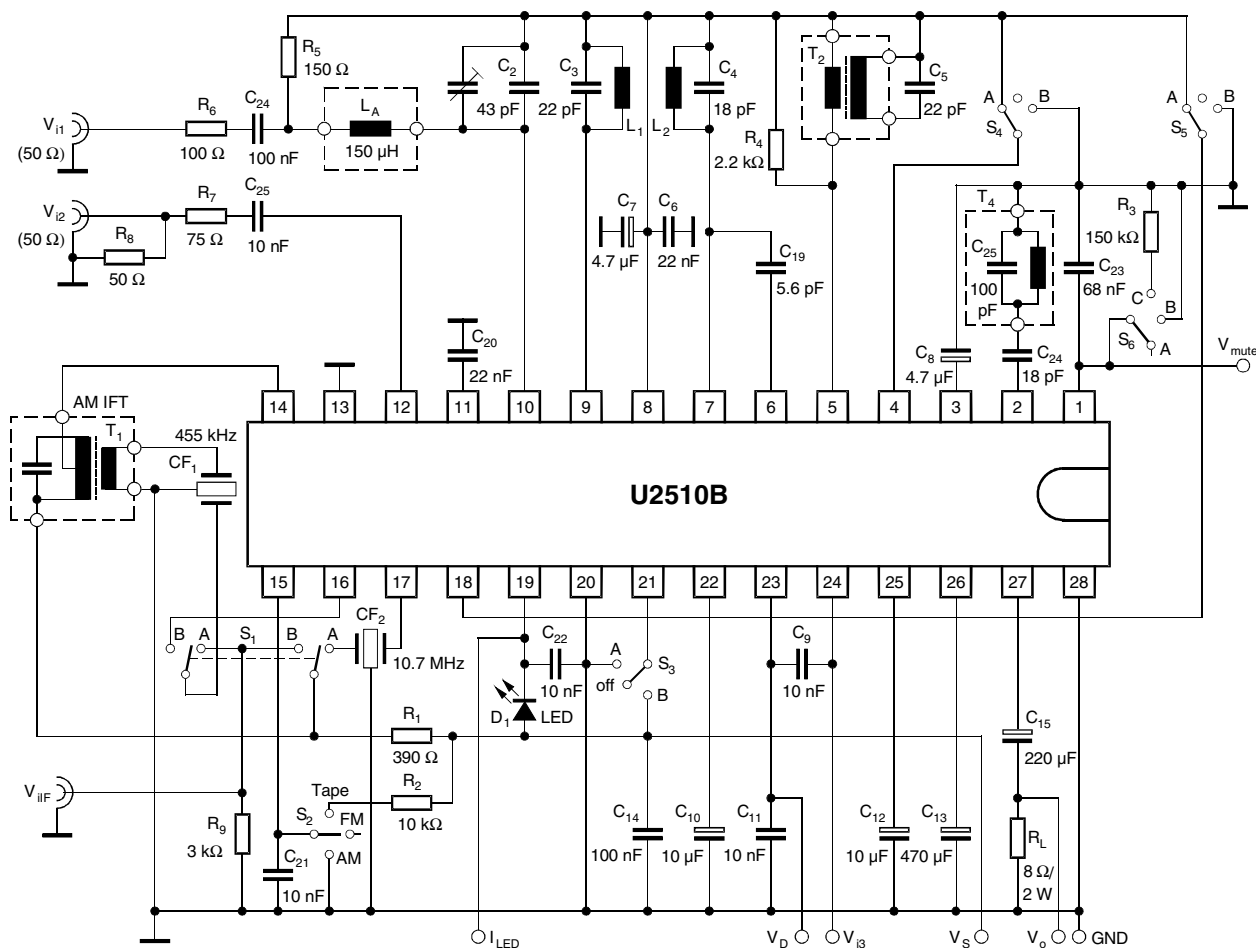
Figure 16. Test Circuit
