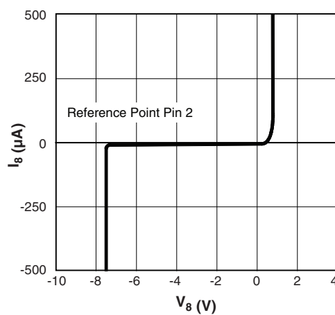
Figure 10-7. f/V Converter Voltage Limitation
