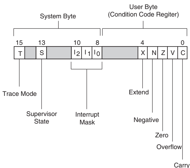
Figure 2-12. Status Register
