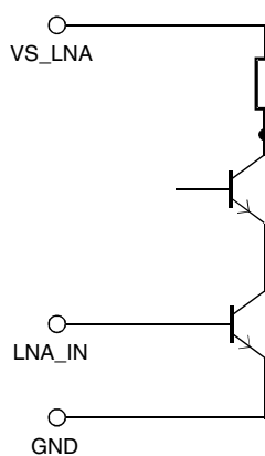
Figure 8-6. Internal Circuitry LNA_IN, VS_LNA
