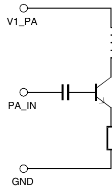
Figure 8-1. Internal Circuitry; PA_IN, V1_PA
