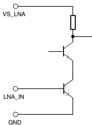
Figure 10-6. Input Circuit LNA_IN/VS_LNA
