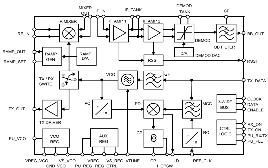
Figure 1. Block Diagram
