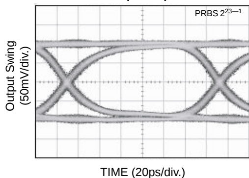
7Gbps Output
