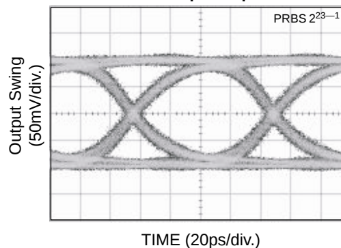
10.7Gbps Output
