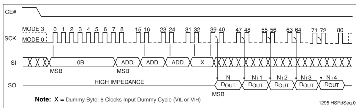
Figure 6: High-Speed-Read Sequence
