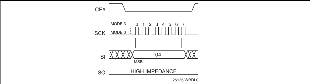
FIGURE 4-17: WRITE DISABLE (WRDI) SEQUENCE
