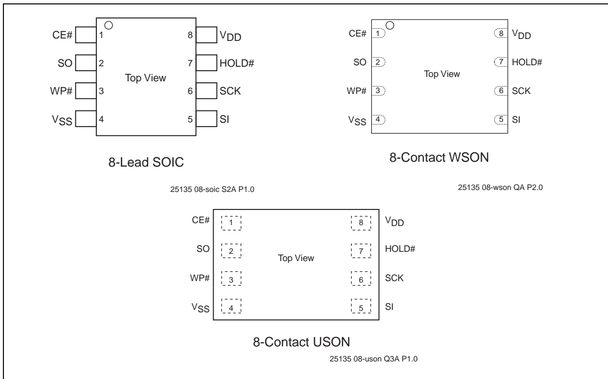
FIGURE 2-1: PIN ASSIGNMENTS
