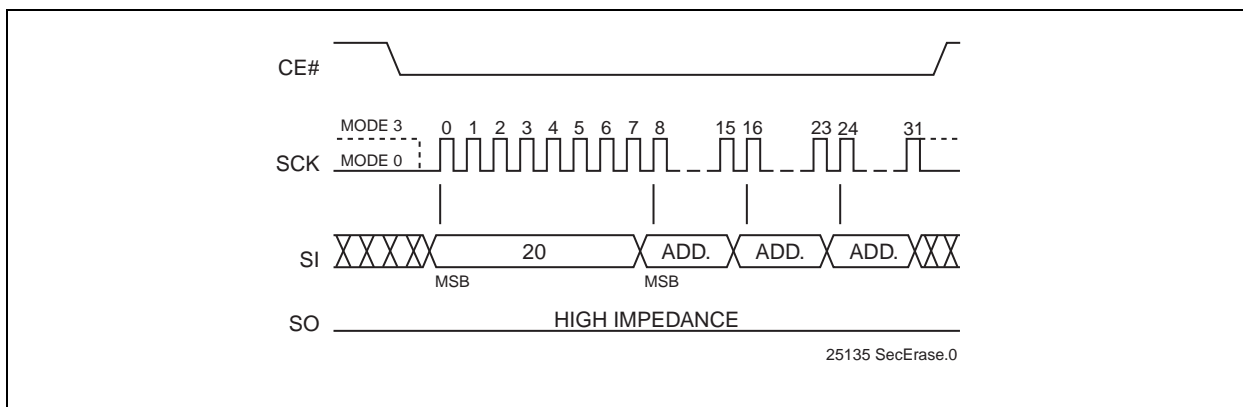
FIGURE 4-10: SECTOR-ERASE SEQUENCE
