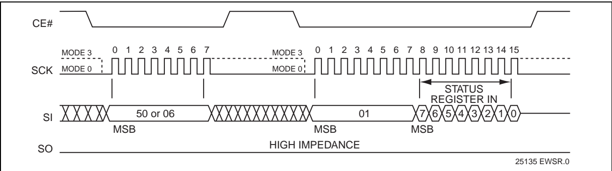
FIGURE 4-18: ENABLE-WRITE-STATUS-REGISTER (EWSR) OR WRITE-ENABLE (WREN) AND WRITE-STATUS-REGISTER (WRSR) BYTE-DATA INPUT SEQUENCE
