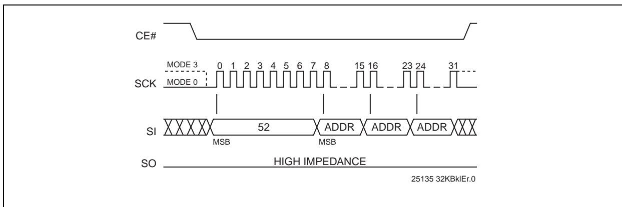
FIGURE 4-11: 32-KBYTE BLOCK-ERASE SEQUENCE
