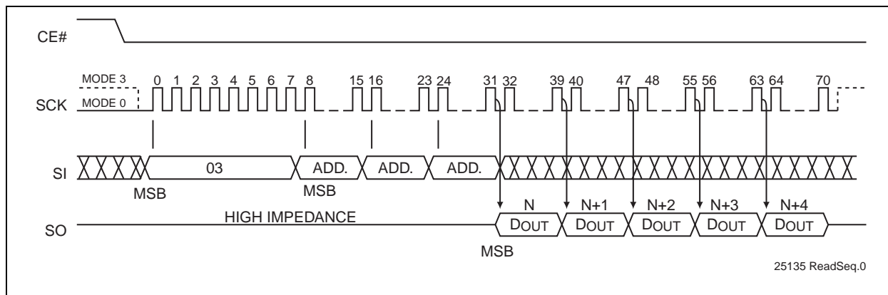
FIGURE 4-3: READ SEQUENCE
