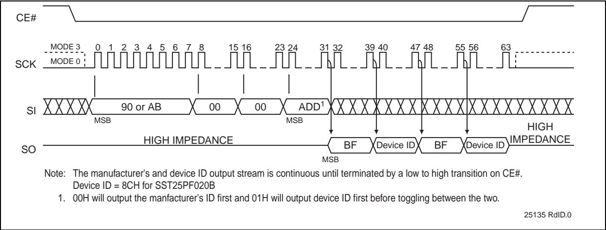
FIGURE 4-21: READ-ID SEQUENCE
