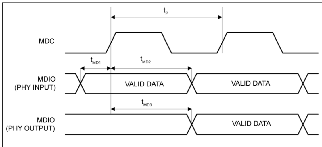
Figure 24. MDC/MDIO Timing
