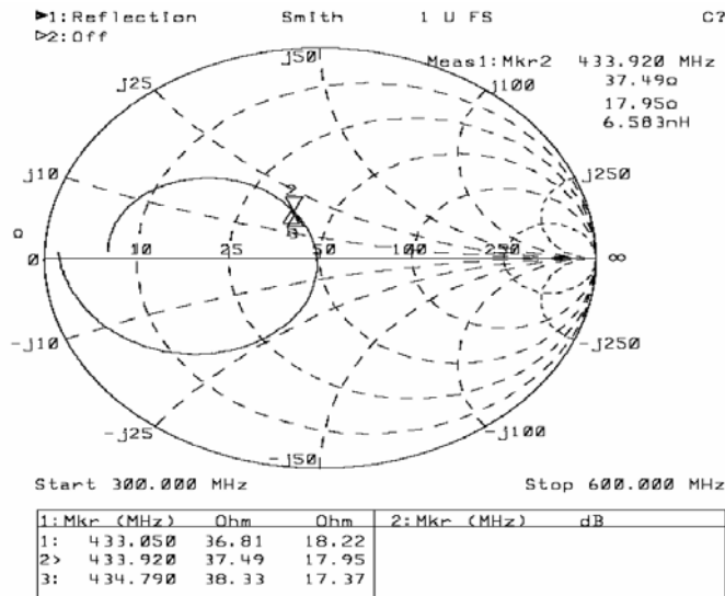
Figure 9. Input Impedance
