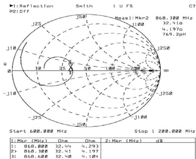
Figure 9. Input Impedance
