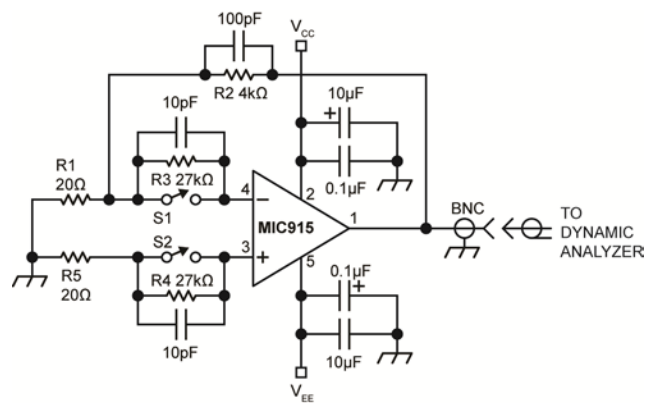
Noise Measurement
