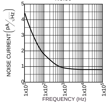
Current Noise
