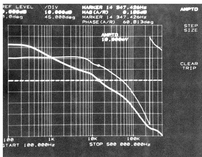
Figure 6b. 5V/2A Output Bode Plot ( \theta margin = 61°)
