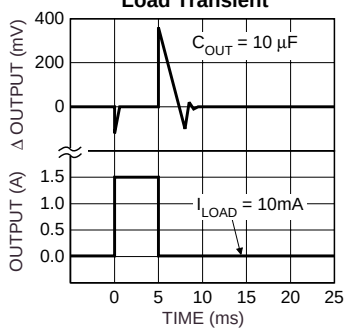
MIC2915x Load Transient
