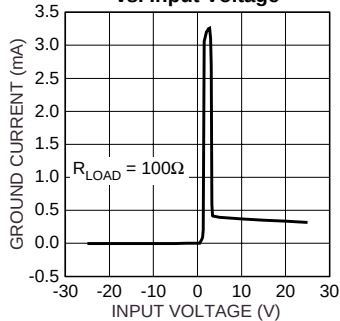
MIC2975x Ground Current vs. Input Voltage
