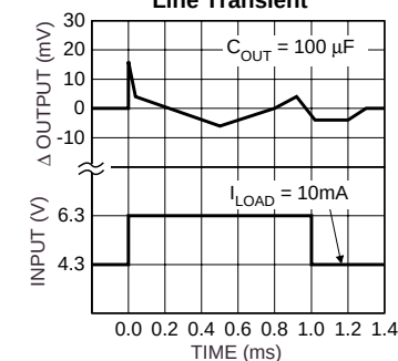
MIC2975x Line Transient
