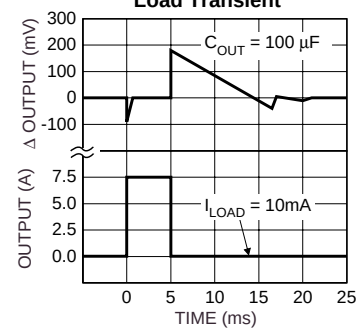
MIC2975x Load Transient
