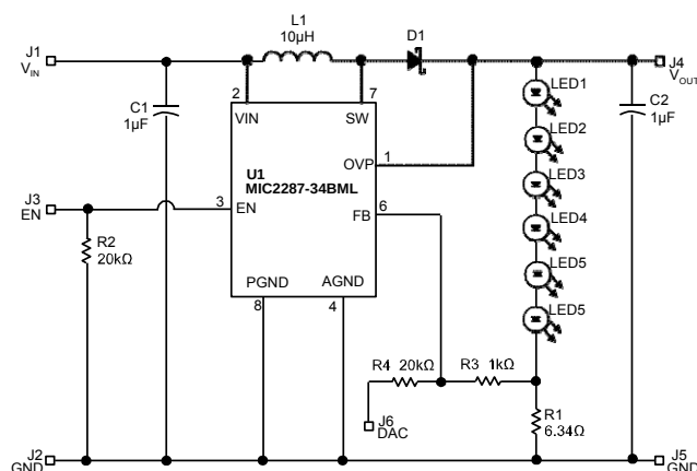
6 LED Configuration
