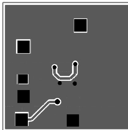
Figure 1d. Bottom Layer
