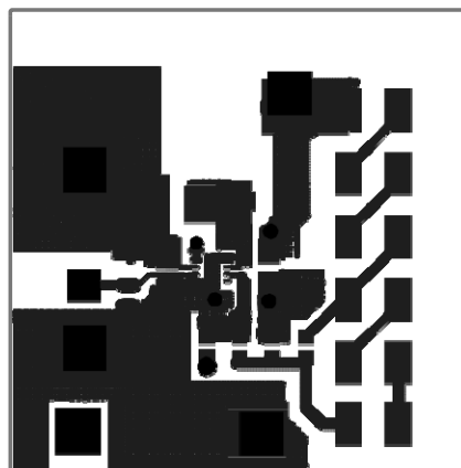
Figure 1b. Top Layer
