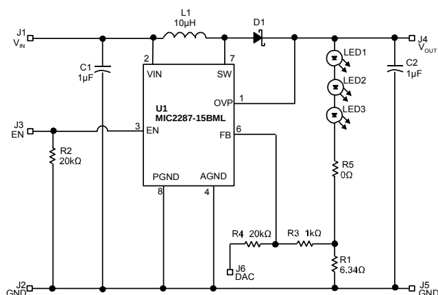
3 LED Configuration
