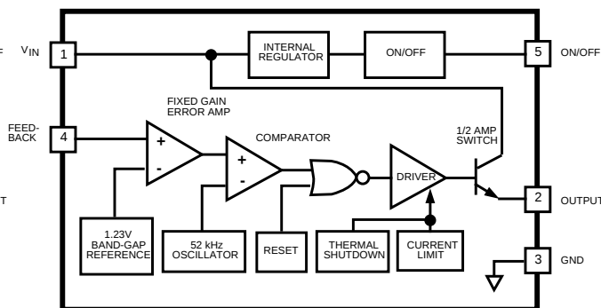
Adjustable Regulator
