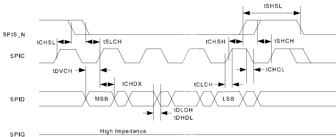
Figure 25. SPI Input Timing
