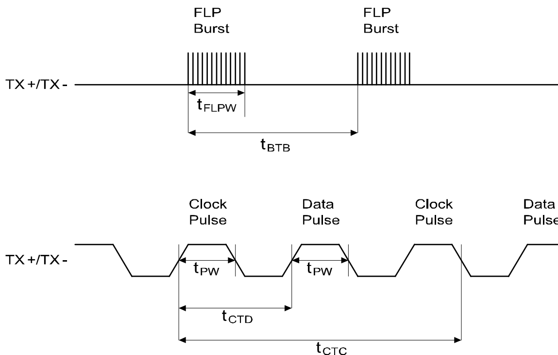
Figure 27. Auto-Negotiation Timing
