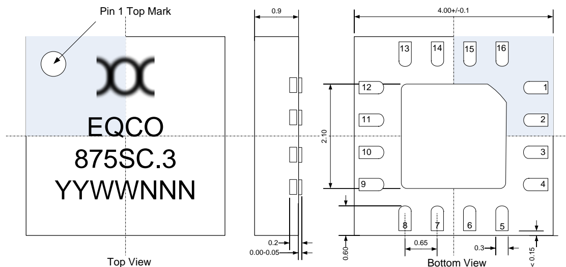
Figure 5: Package Drawing
