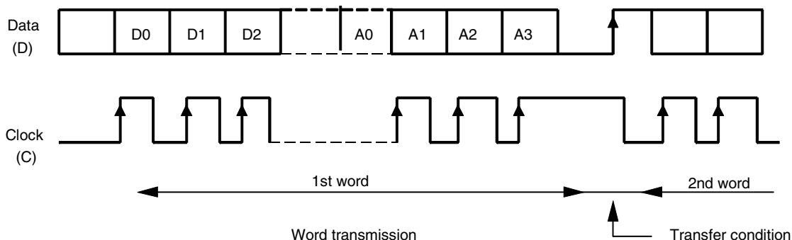
Figure 3-2. Serial Bus Transmission
