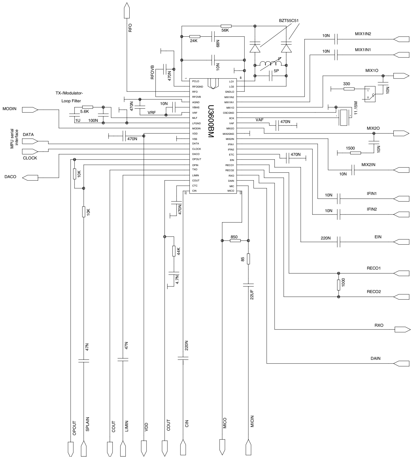
Figure 8-1. Test Circuit
