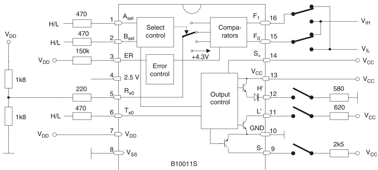
Figure 6-2. Application Circuit
