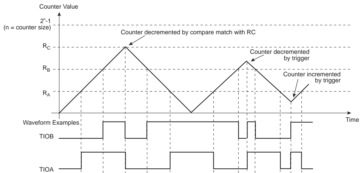
Figure 31-15. WAVSEL = 11 with Trigger
