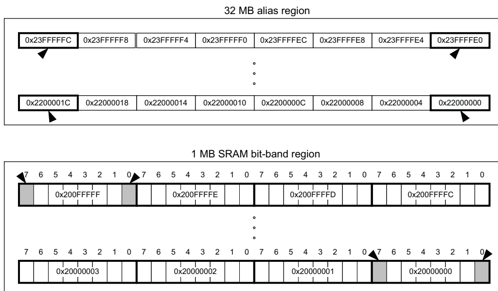
Figure 10-4. Bit-band Mapping
