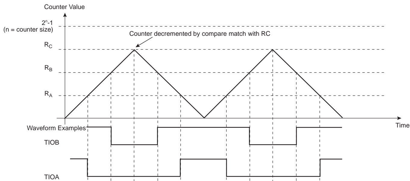
Figure 31-14. WAVSEL = 11 without Trigger
