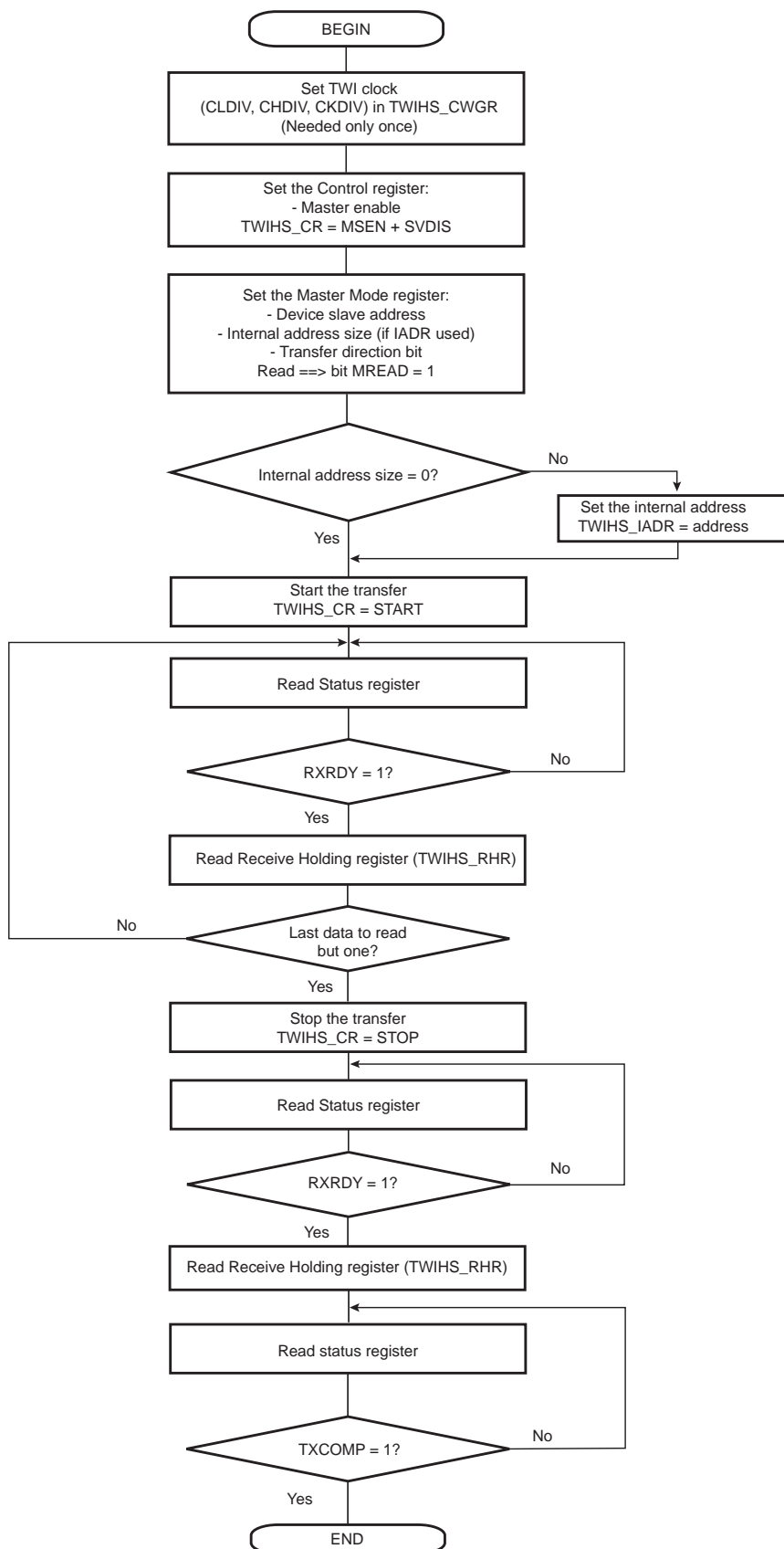
Figure 27-26. TWI Read Operation with Multiple Data Bytes with or without Internal Address
