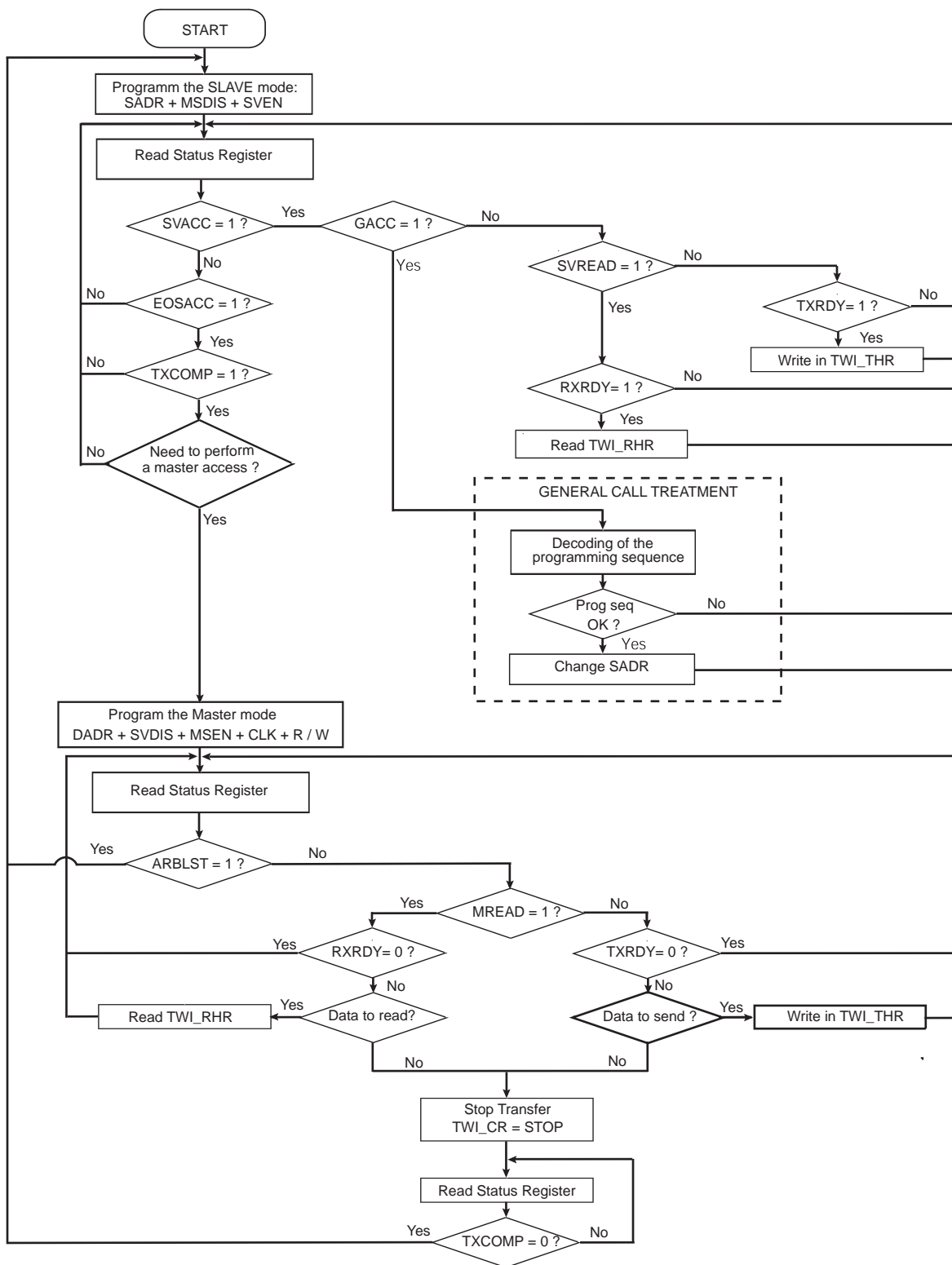
Figure 28-24. Multi-master Flowchart
