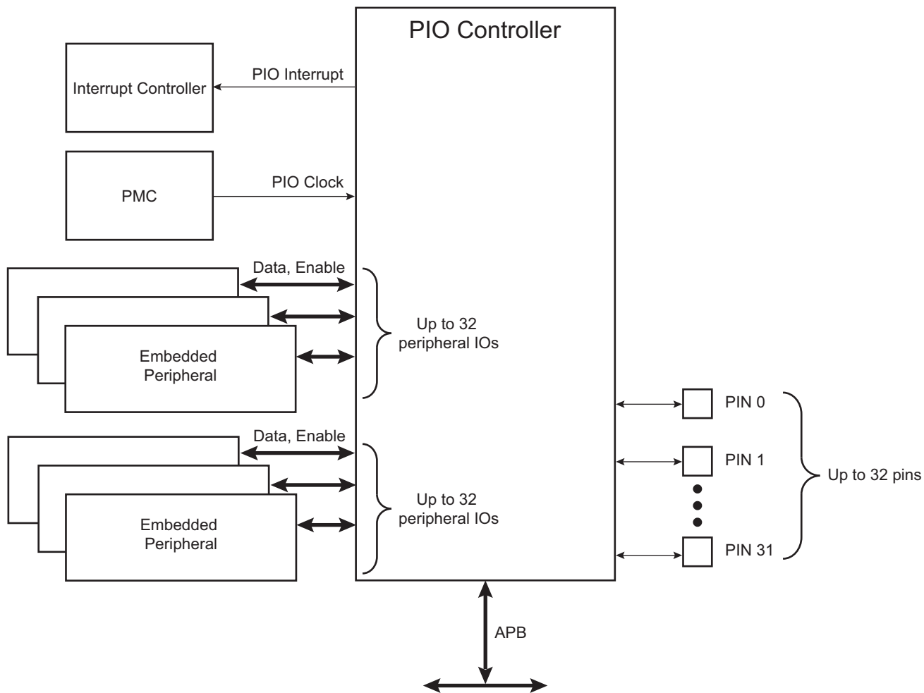
Figure 25-1. Block Diagram
