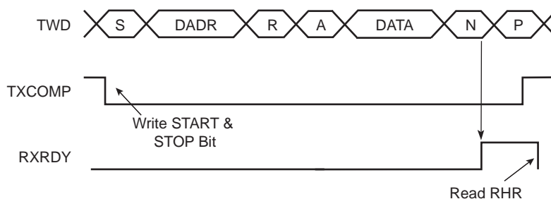
Figure 27-10. Master Read with One Data Byte
