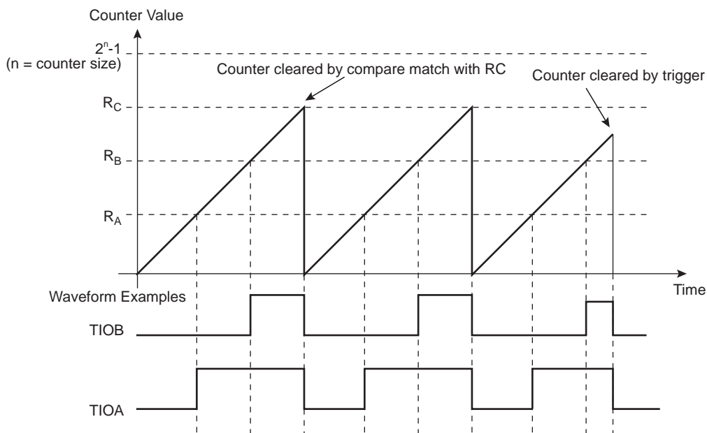
Figure 31-11. WAVSEL = 10 with Trigger
