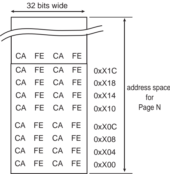
Before programming: Unerased page in Flash array
