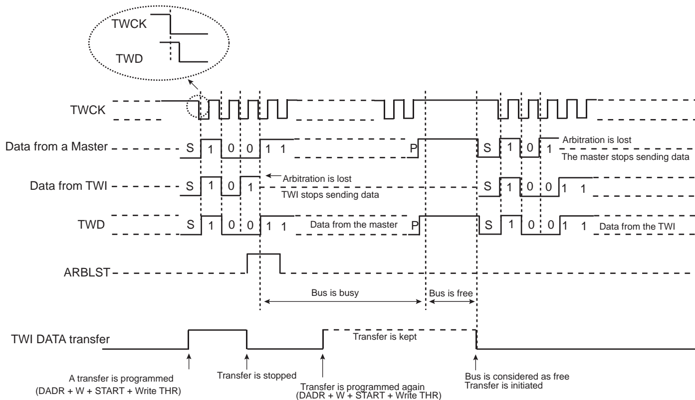
Figure 28-23. Arbitration Cases
