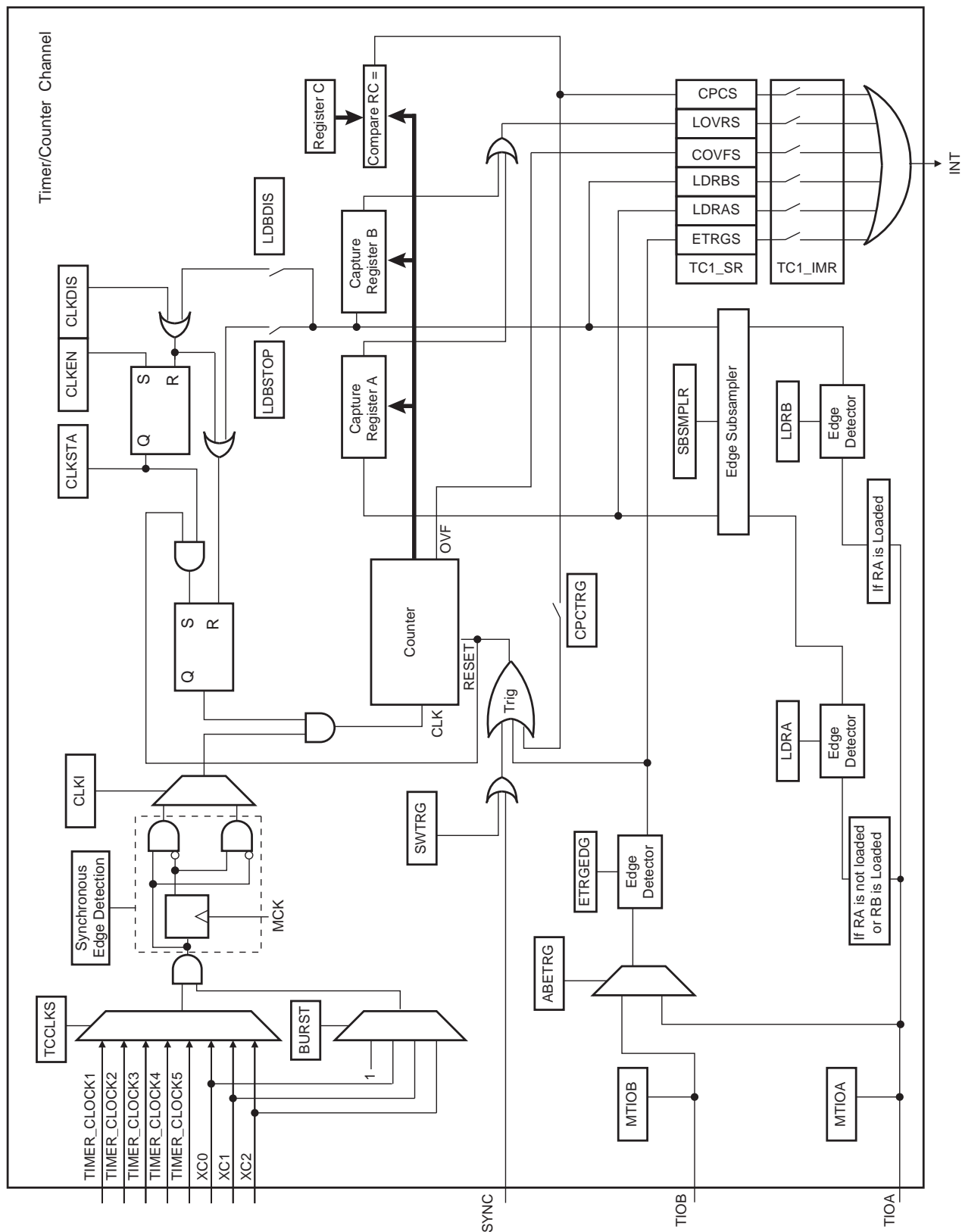
Figure 31-6. Capture Mode
