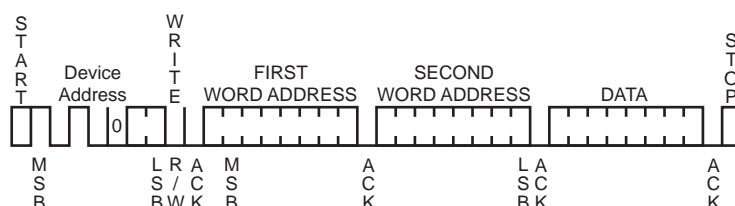
Figure 27-15. Internal Address Usage
