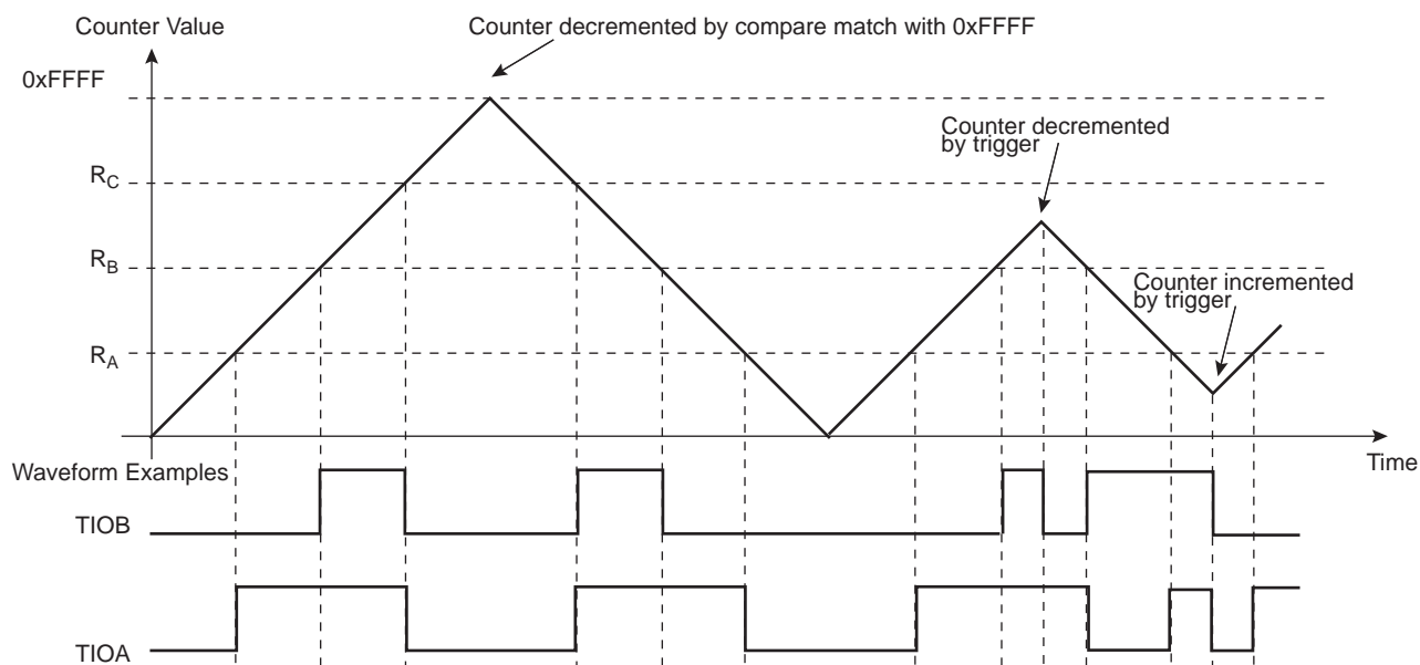
Figure 31-13. WAVSEL = 01 with Trigger
