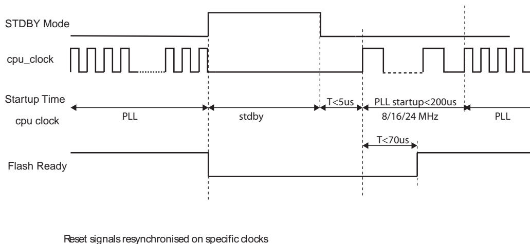
Figure 5-3. Start-up Sequence
