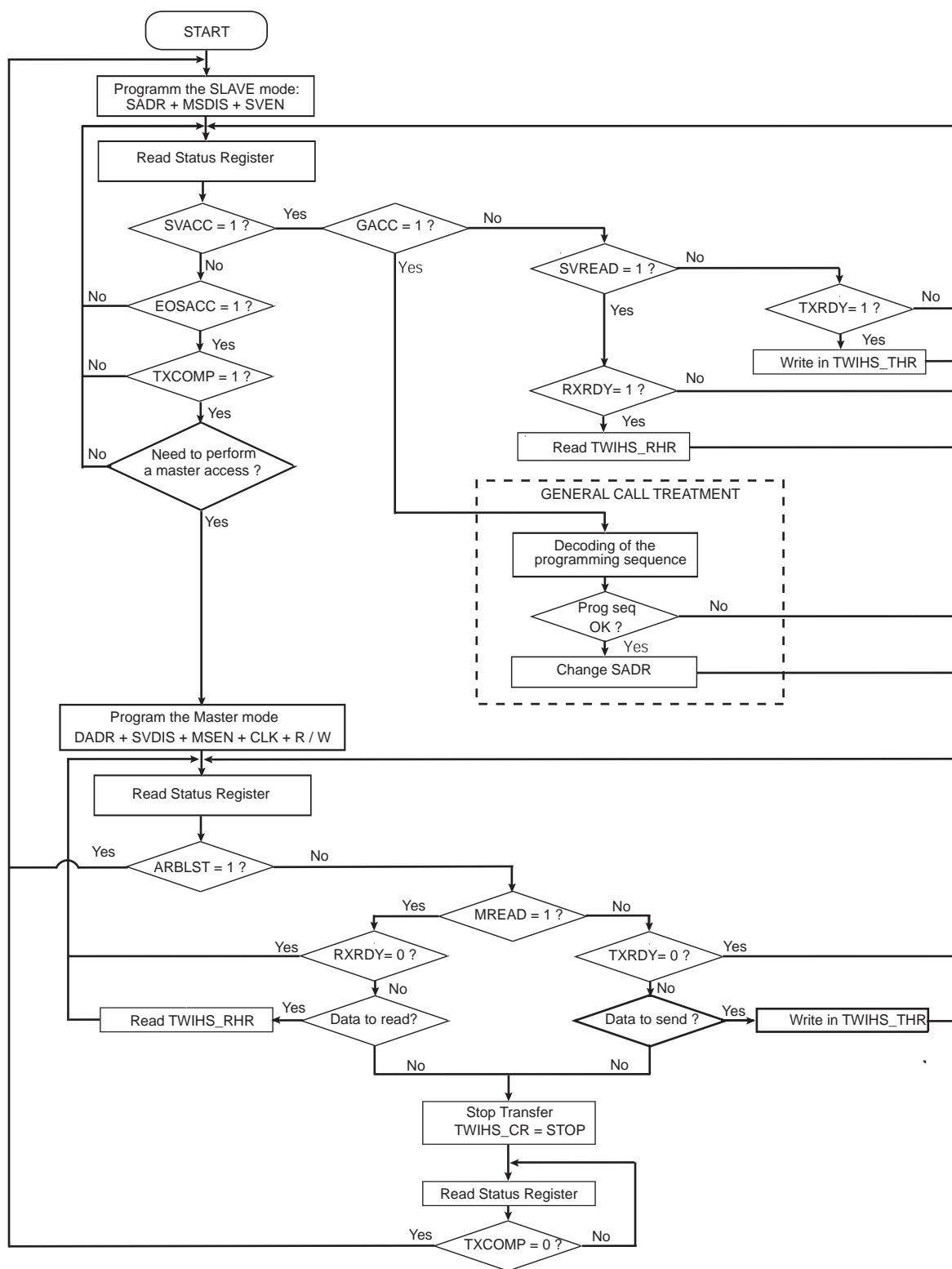
Figure 27-33. Multi-Master Flowchart
