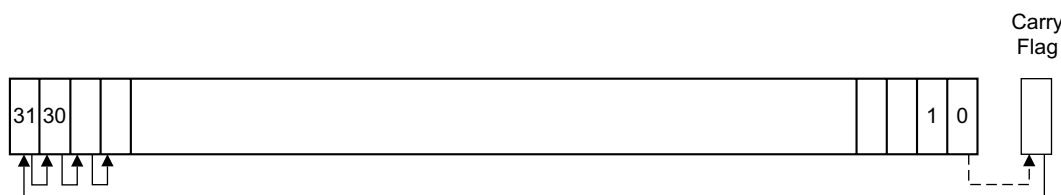
Figure 10-12. RRX
