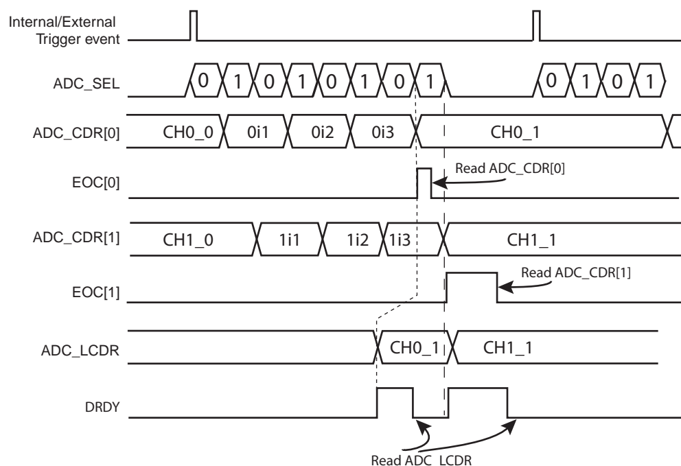
Figure 32-10. Digital Averaging Function Waveforms on a Single Trigger Event
