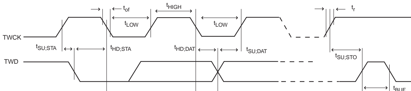
Figure 33-16. Two-wire Serial Bus Timing
