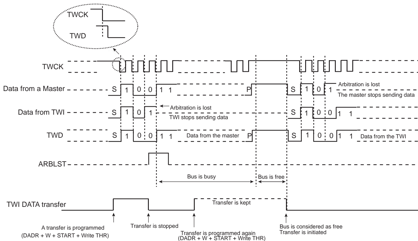
Figure 27-32. Arbitration Cases
