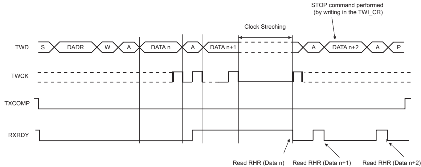
Figure 28-11. Master Read Clock Stretching with Multiple Data Bytes
