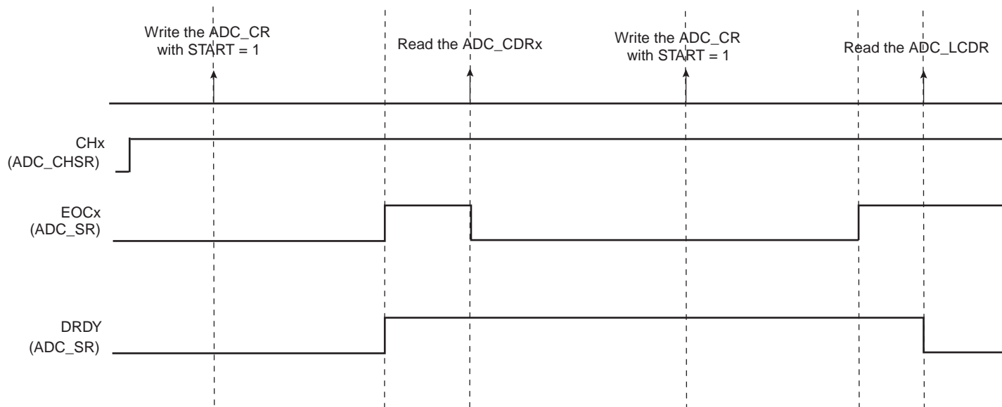
Figure 32-3. EOCx and DRDY Flag Behavior
