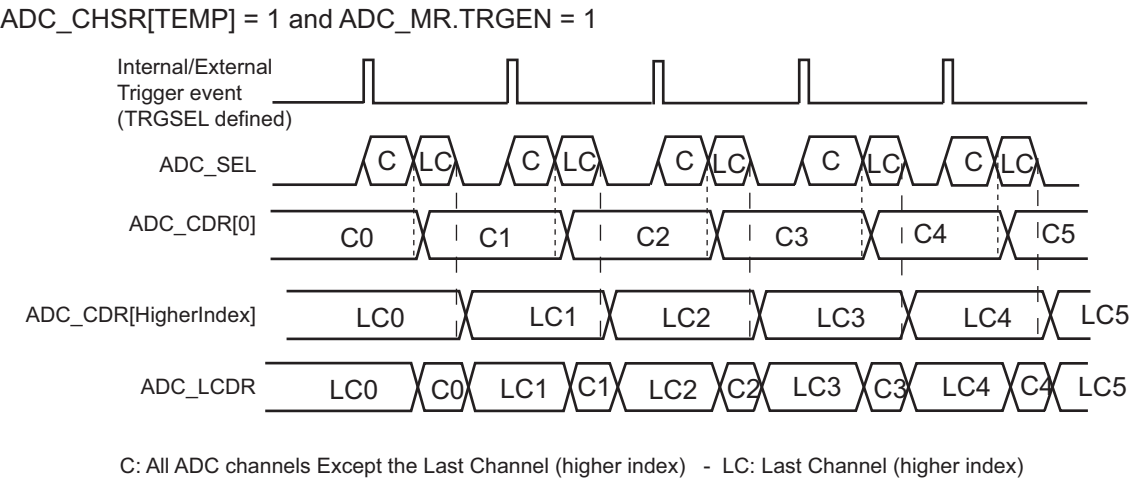
Figure 32-6. Same Trigger for All Channels
