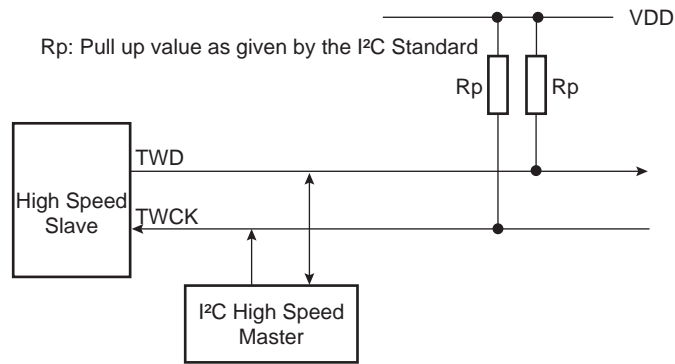
Figure 27-2. High-Speed Mode Application Block Diagram
