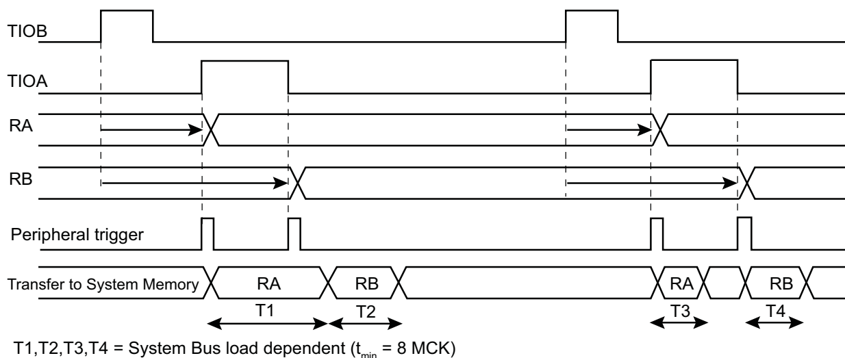
Figure 31-5. Example of Transfer with PDC
