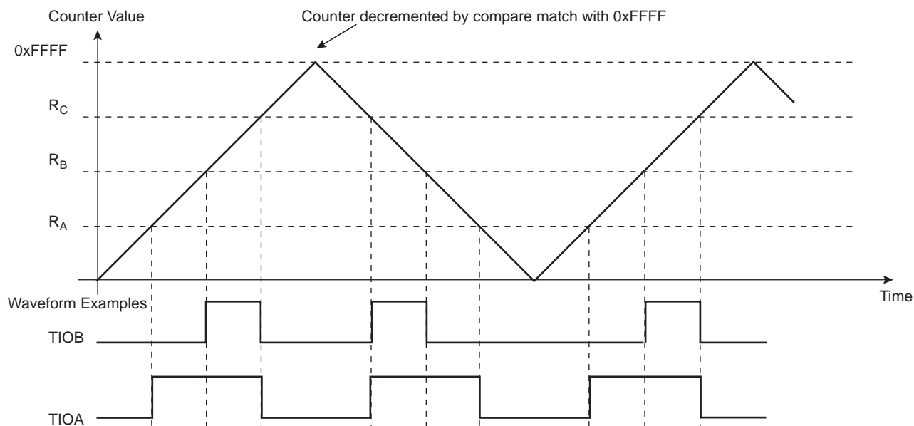
Figure 31-12. WAVSEL = 01 without Trigger
