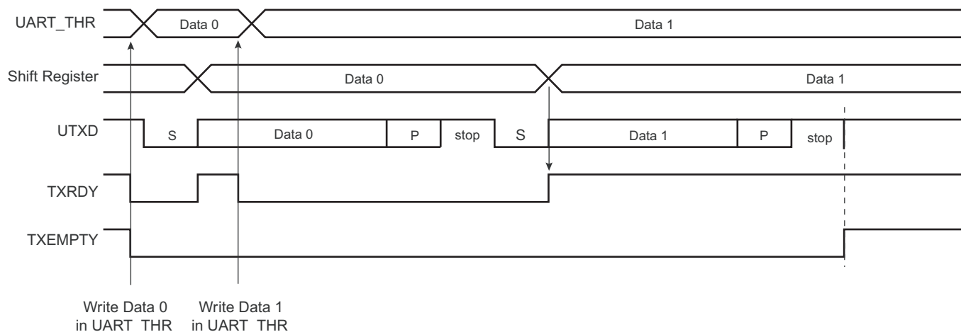
Figure 29-10. Transmitter Control
