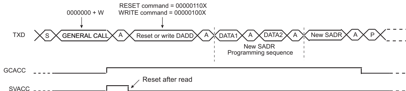
Figure 28-28. Master Performs a General Call
