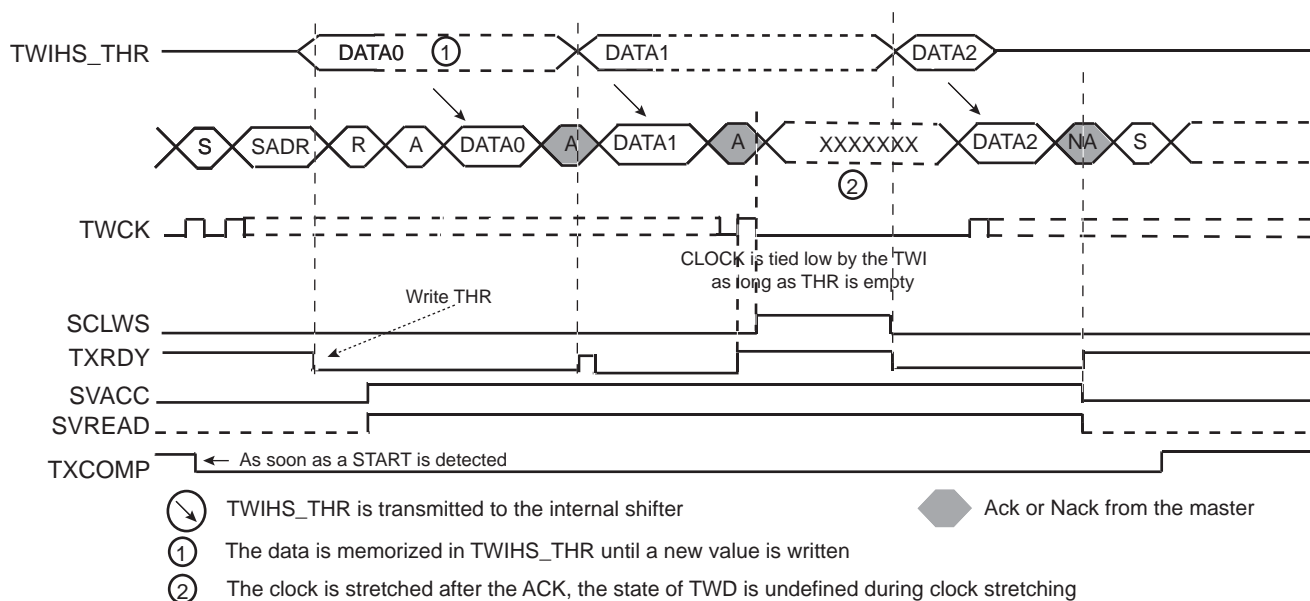
Figure 27-39. Clock Stretching in Read Mode
