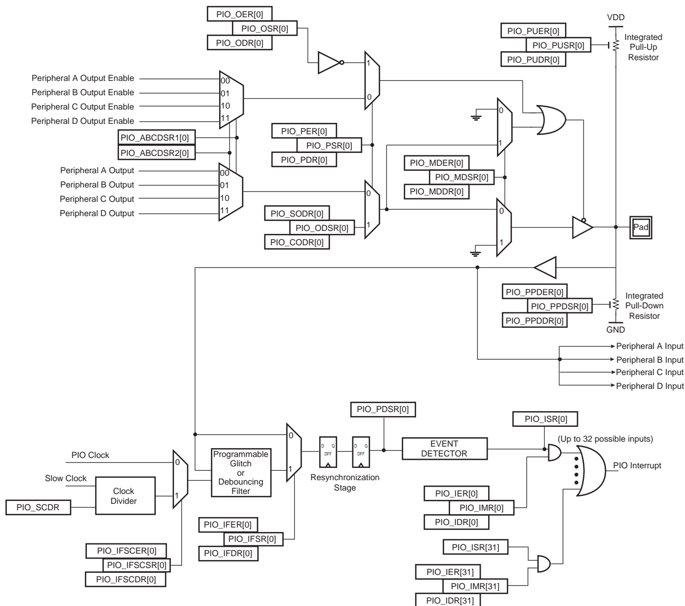
Figure 25-3. I/O Line Control Logic
