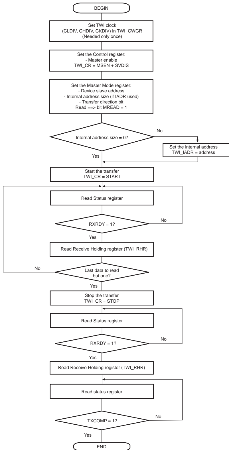
Figure 28-21. TWI Read Operation with Multiple Data Bytes with or without Internal Address
