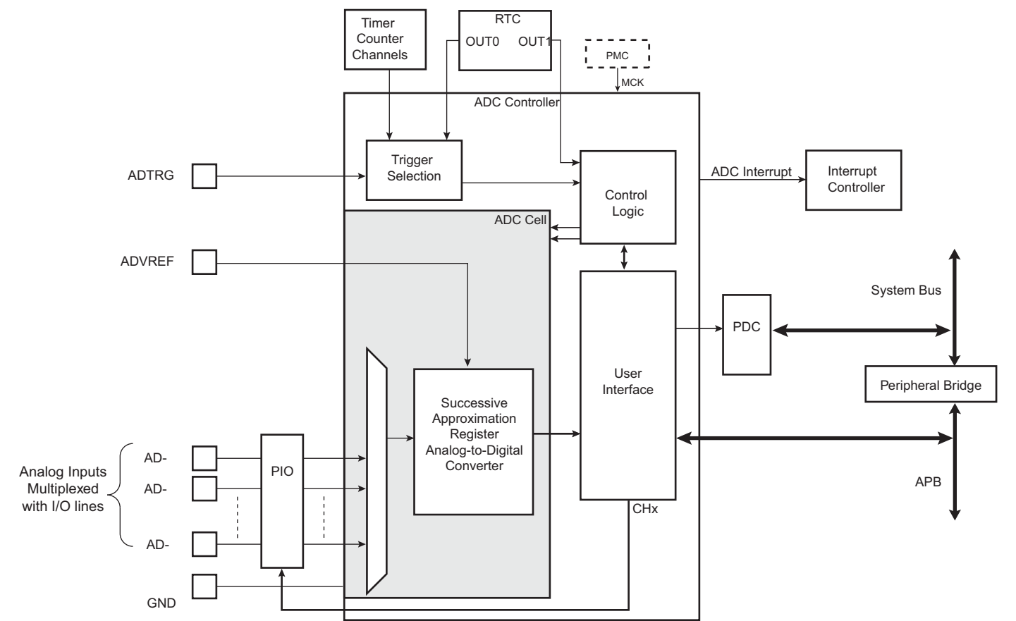
Figure 32-1. Analog-to-Digital Converter Block Diagram
