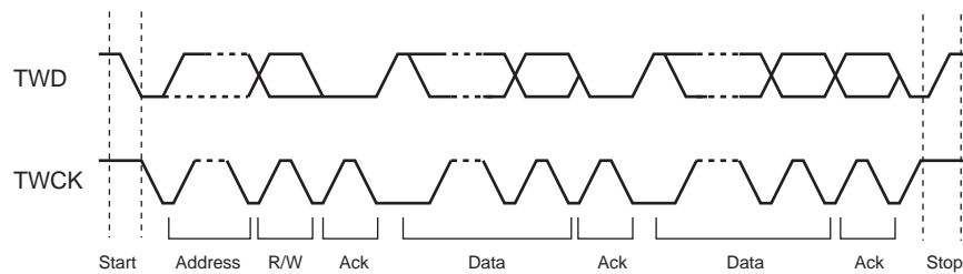
Figure 27-5. Transfer Format
