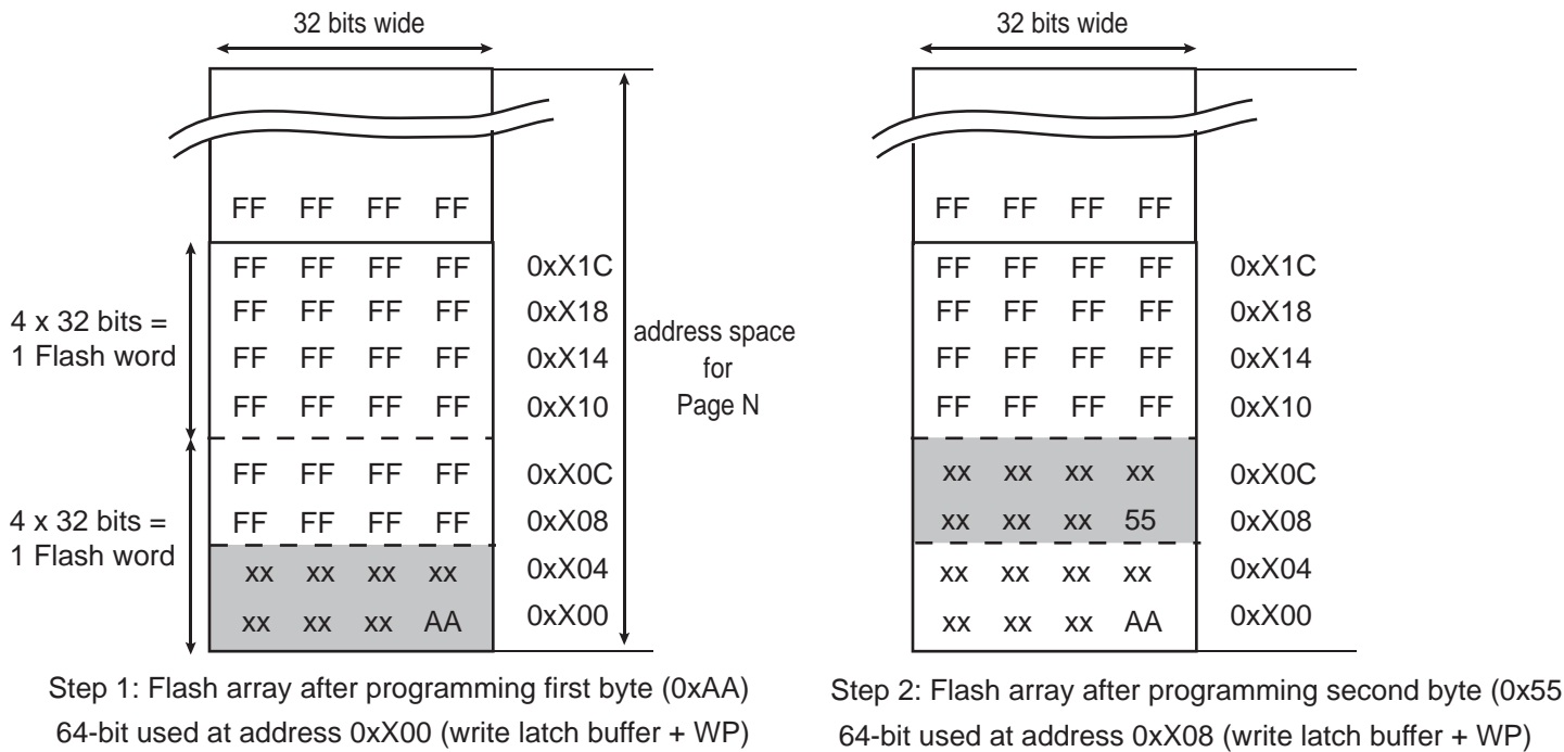
Figure 19-10. Programming Bytes in the Flash
