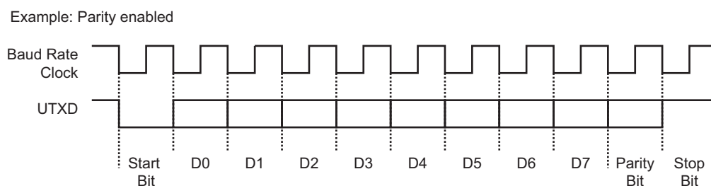
Figure 29-9. Character Transmission
