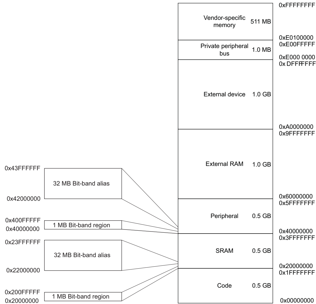
Figure 10-3. Memory Map
