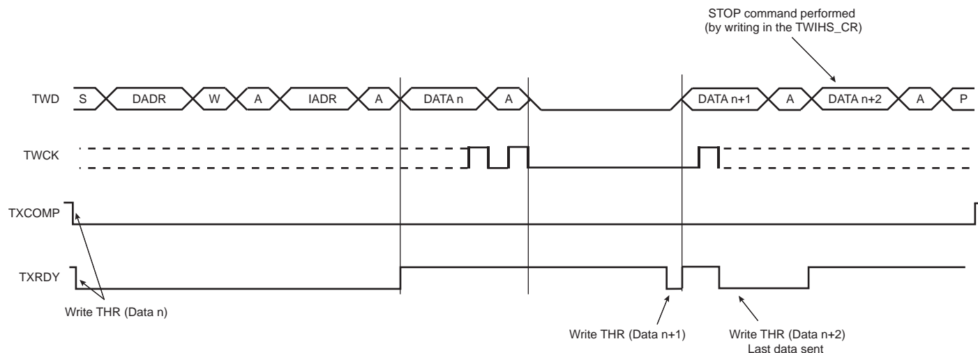
Figure 27-9. Master Write with One Byte Internal Address and Multiple Data Bytes
