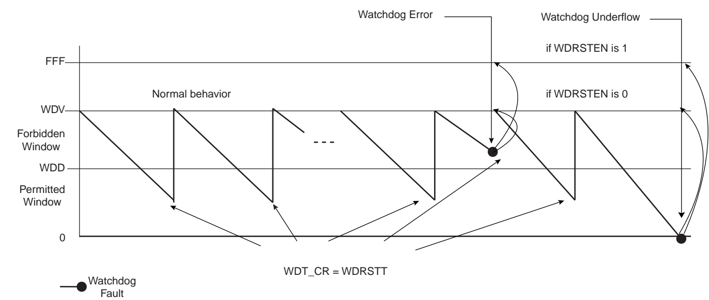
Figure 15-2. Watchdog Behavior
