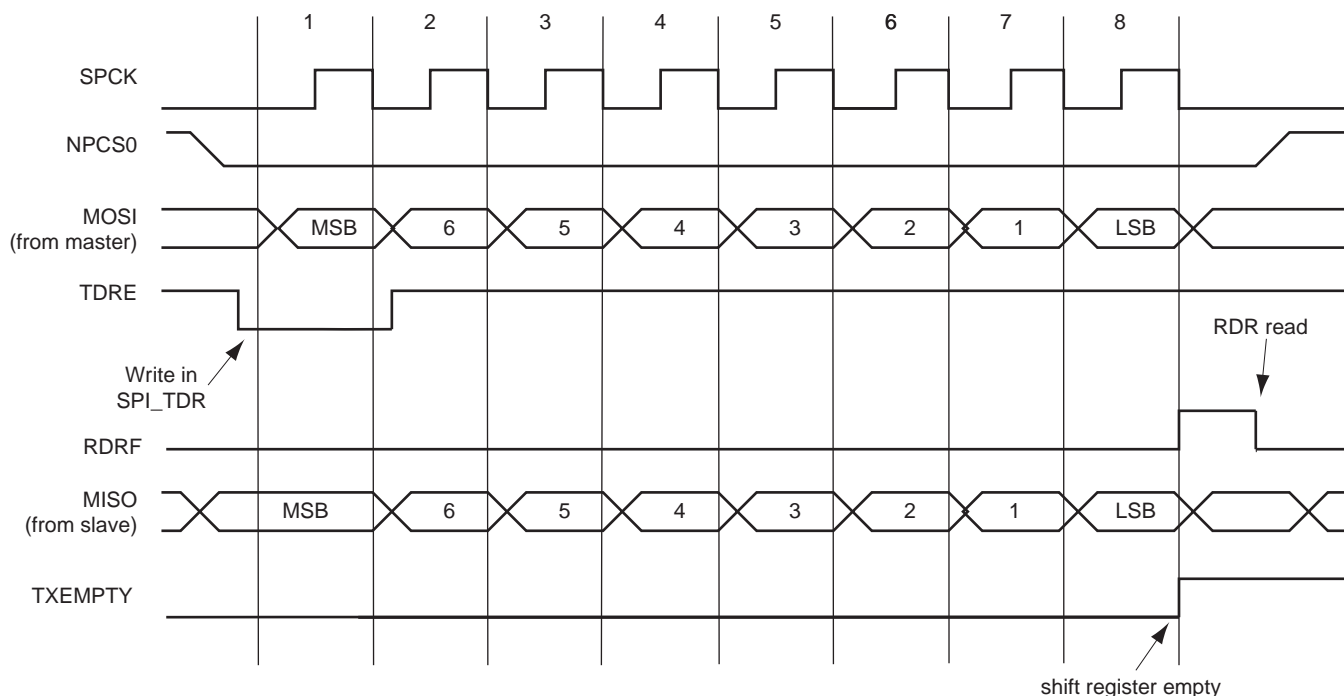
Figure 26-7. Status Register Flags Behavior
