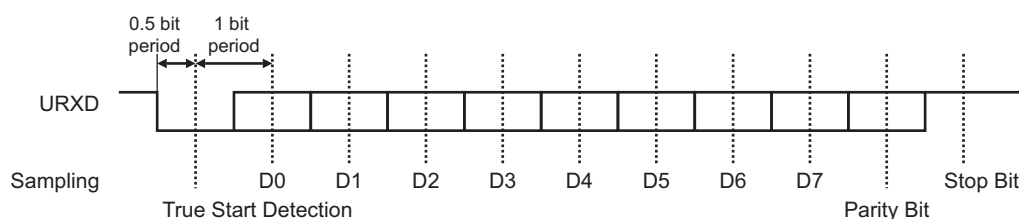
Figure 29-4. Character Reception
