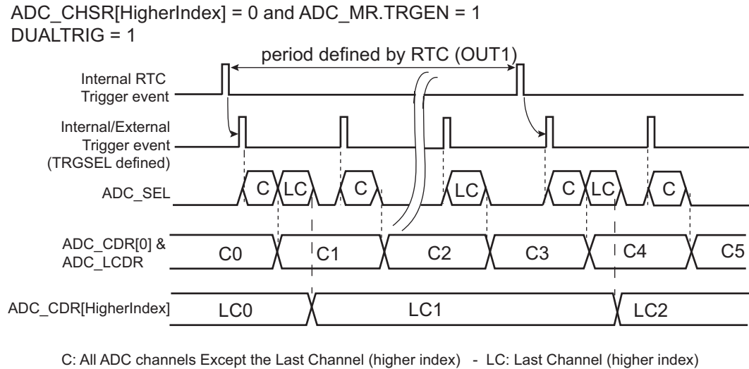
Figure 32-7. Independent Trigger Measurement for Last Channel
