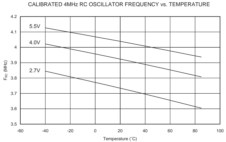
Figure 173. Calibrated 4 MHz RC Oscillator Frequency vs. Temperature
