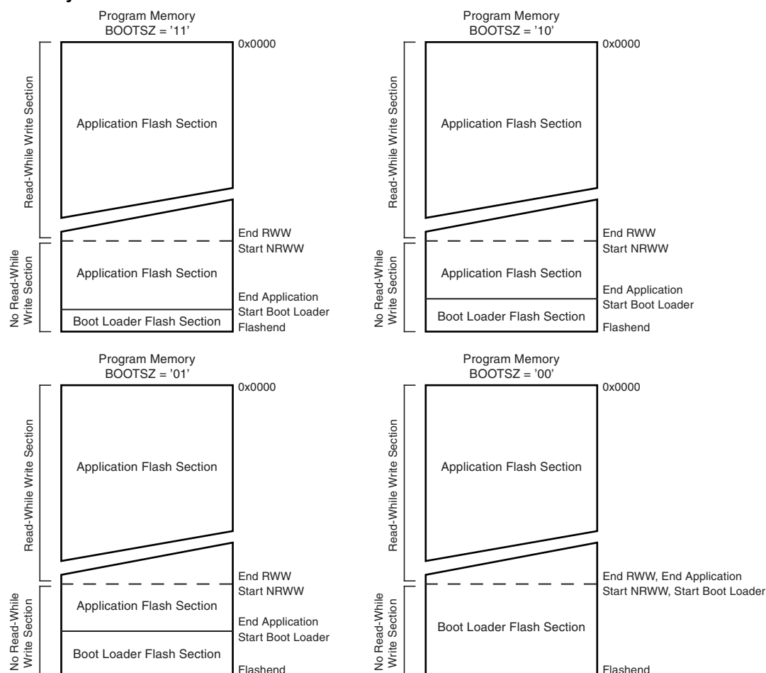
Figure 29-2. Memory Sections
