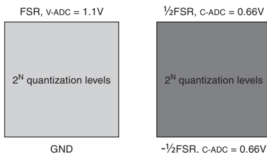
Figure 26-2. Internal Signal Range with VREF = 1.1V
