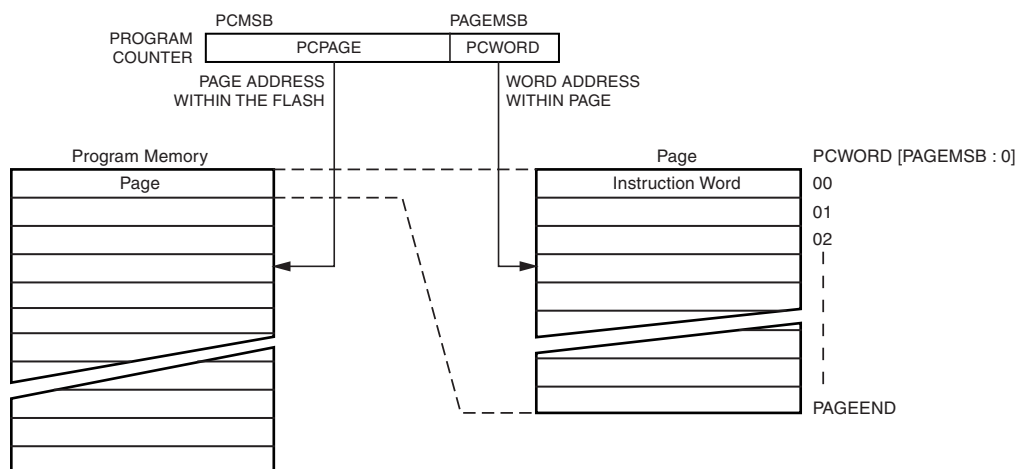
Figure 30-4. Addressing the Flash which is Organized in Pages
