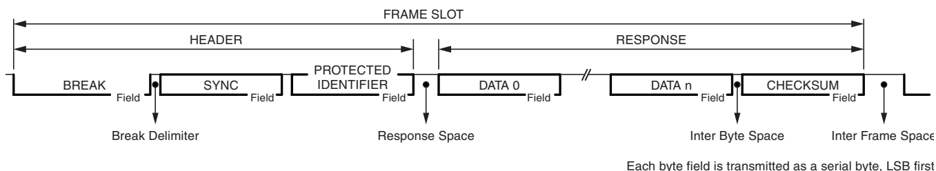
Figure 25-3. Structure of a LIN Frame
