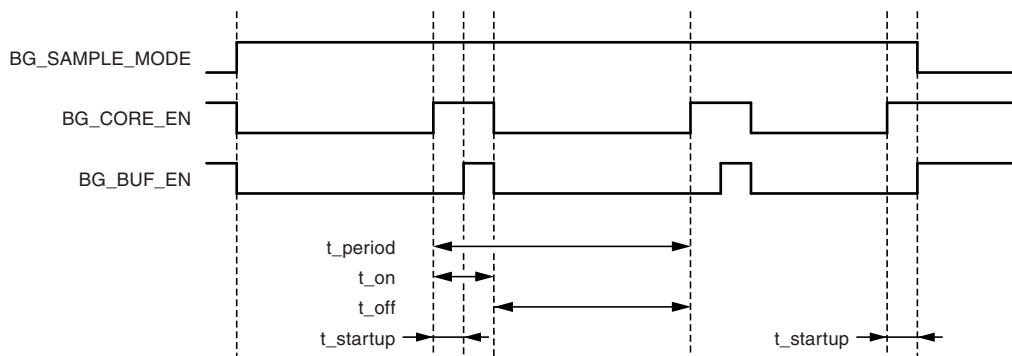
Figure 27-2. Band Gap Timing
