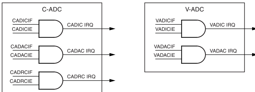
Figure 26-12.ADC Interrupts
