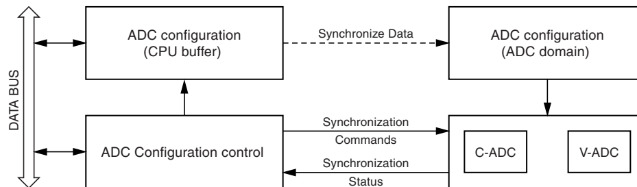
Figure 26-11. Synchronization of Configuration Settings
