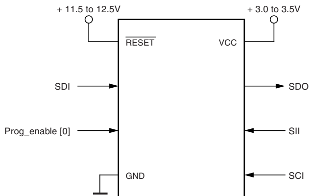
Figure 30-3. High-voltage Serial Programming
