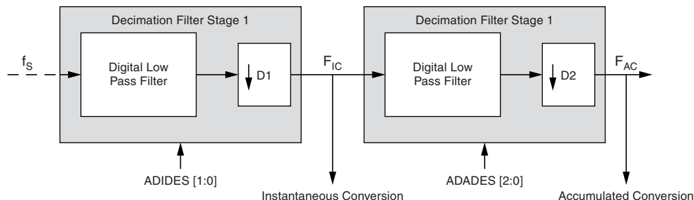
Figure 26-3. Decimation Filter
