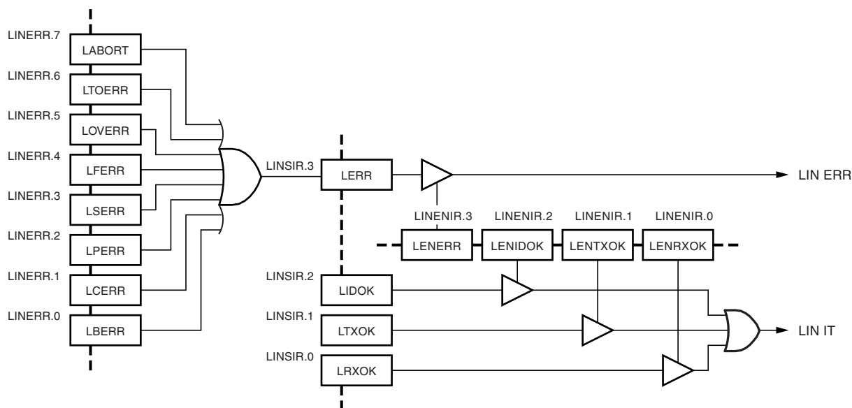
Figure 25-13. LIN Interrupt Mapping
