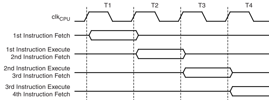
Figure 13-4. The Parallel Instruction Fetches and Instruction Executions
