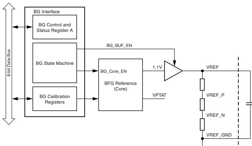
Figure 27-1. Reference Circuitry
