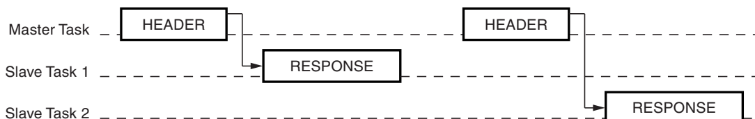
Figure 25-2. Master and Slave Tasks Behavior in LIN Frame
