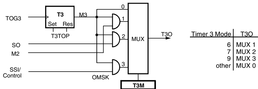
Figure 5-36. Modulator 3
