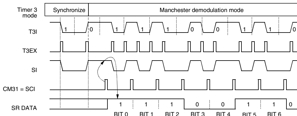
Figure 5-33. Manchester Demodulation
