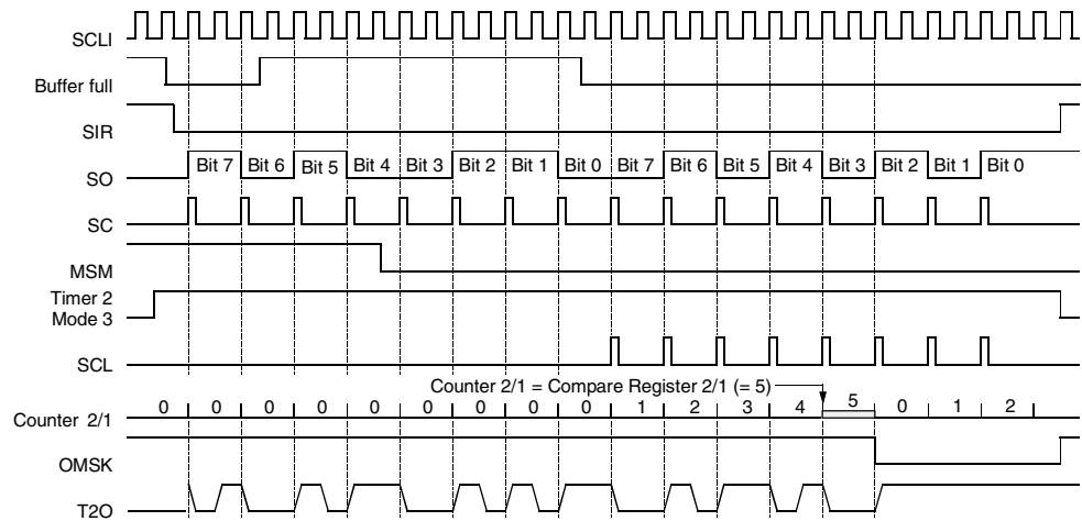
Figure 5-53. Bi-phase Modulation 2
