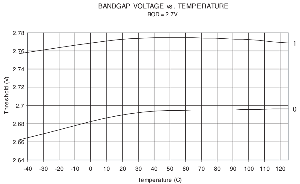
Figure 30-30. BOD Threshold vs, Temperature (BODLEVEL is 2.7V)
