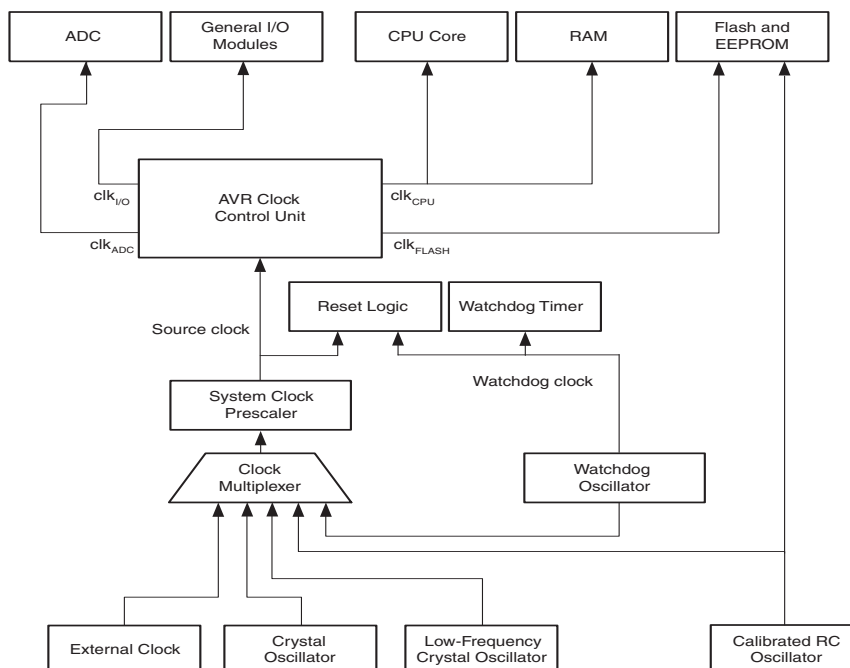
Figure 14-1. Clock Distribution
