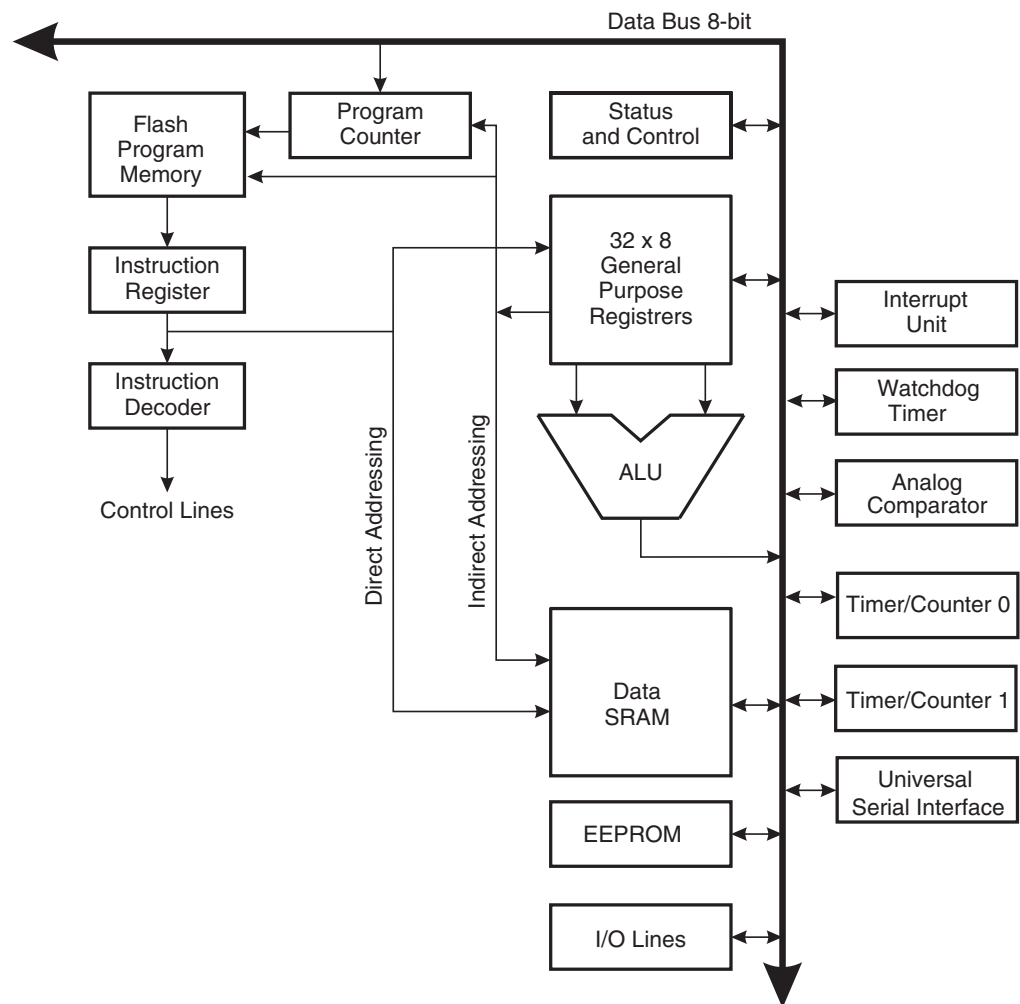
Figure 12-1. Block Diagram of the AVR Architecture
