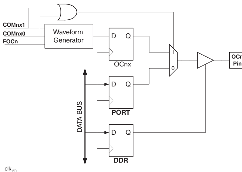
Figure 20-4. Compare Match Output Unit, Schematic
