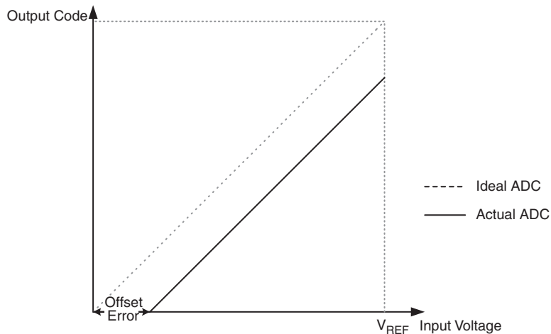
Figure 25-9. Offset Error
