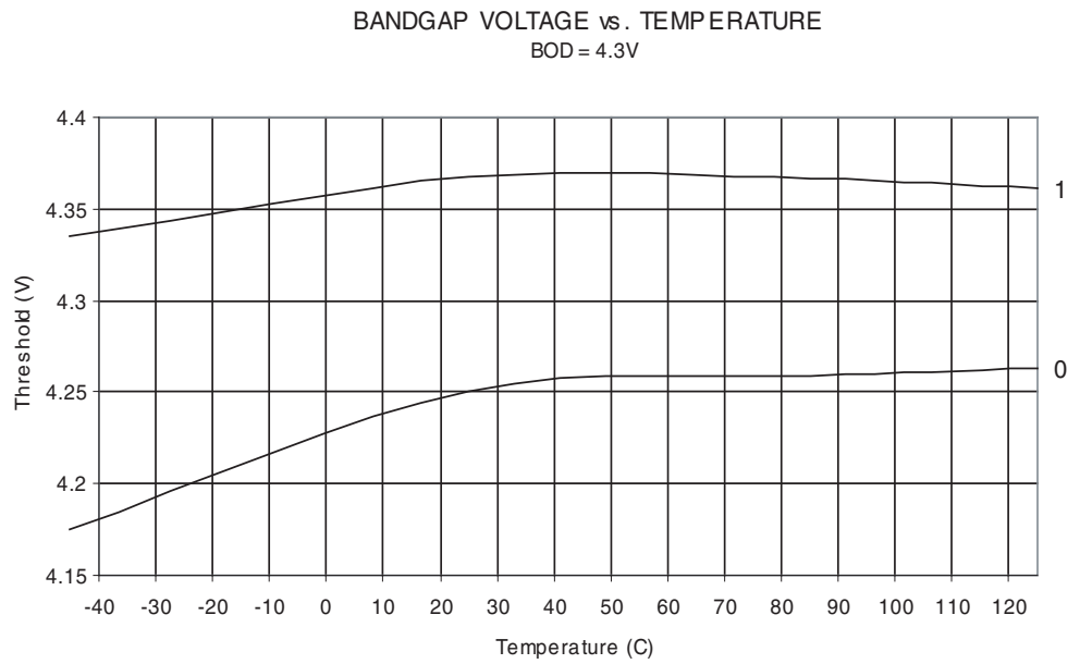
Figure 30-29. BOD Threshold vs. Temperature (BODLEVEL is 4.3V)
