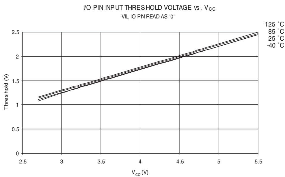
Figure 30-24. I/O Pin Input threshold Voltage vs. V_{CC} ( V_{IL} , IO Pin Read as '0')
