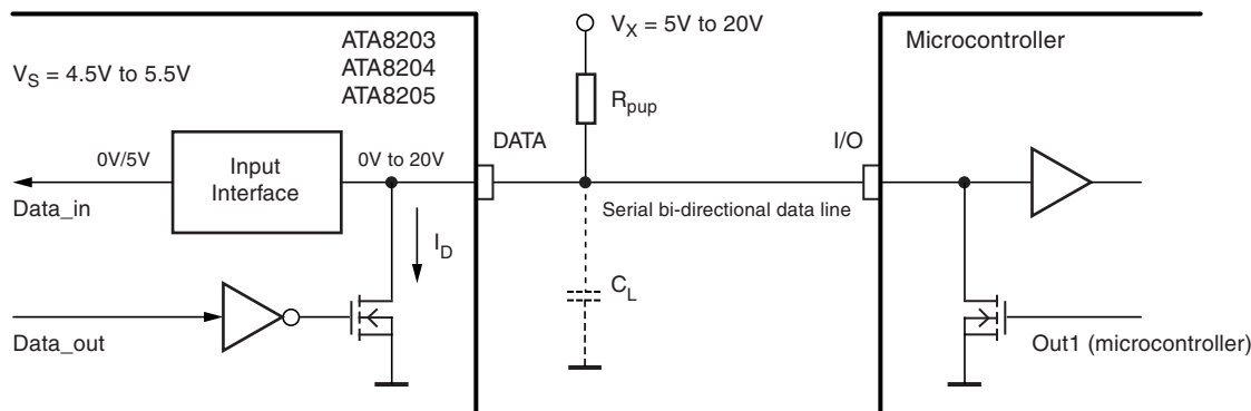
Figure 13-2. Data Interface
