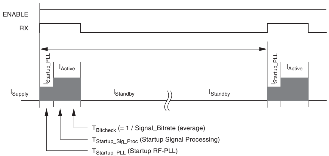
Figure 8-1. Polling Cycle
