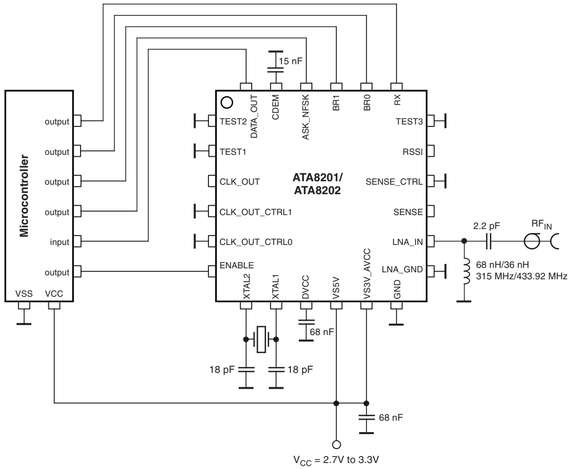
Figure 9-1. 3V Application
