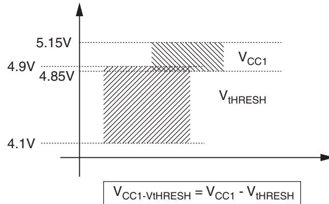
Figure 3-2. Correlation between VCC Output Voltage and Reset Threshold
