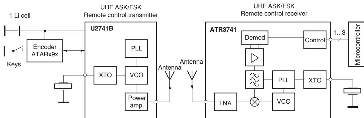
Figure 1-2. Block Diagram
