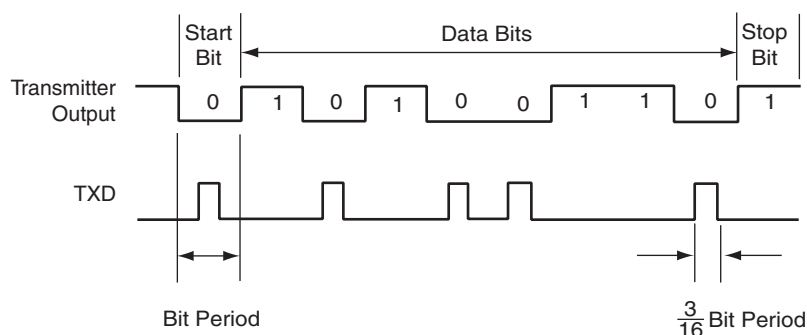
Figure 34-34. IrDA Modulation
