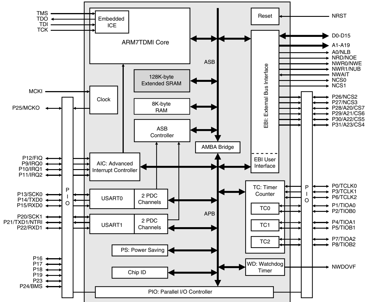
Figure 2. AT91R40807
