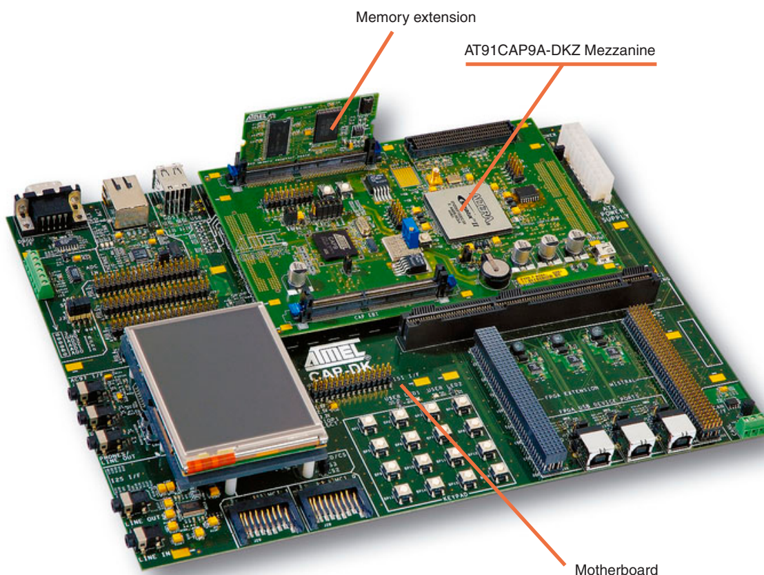
Figure 5-1. AT91CAP9A-DKZ Overview
