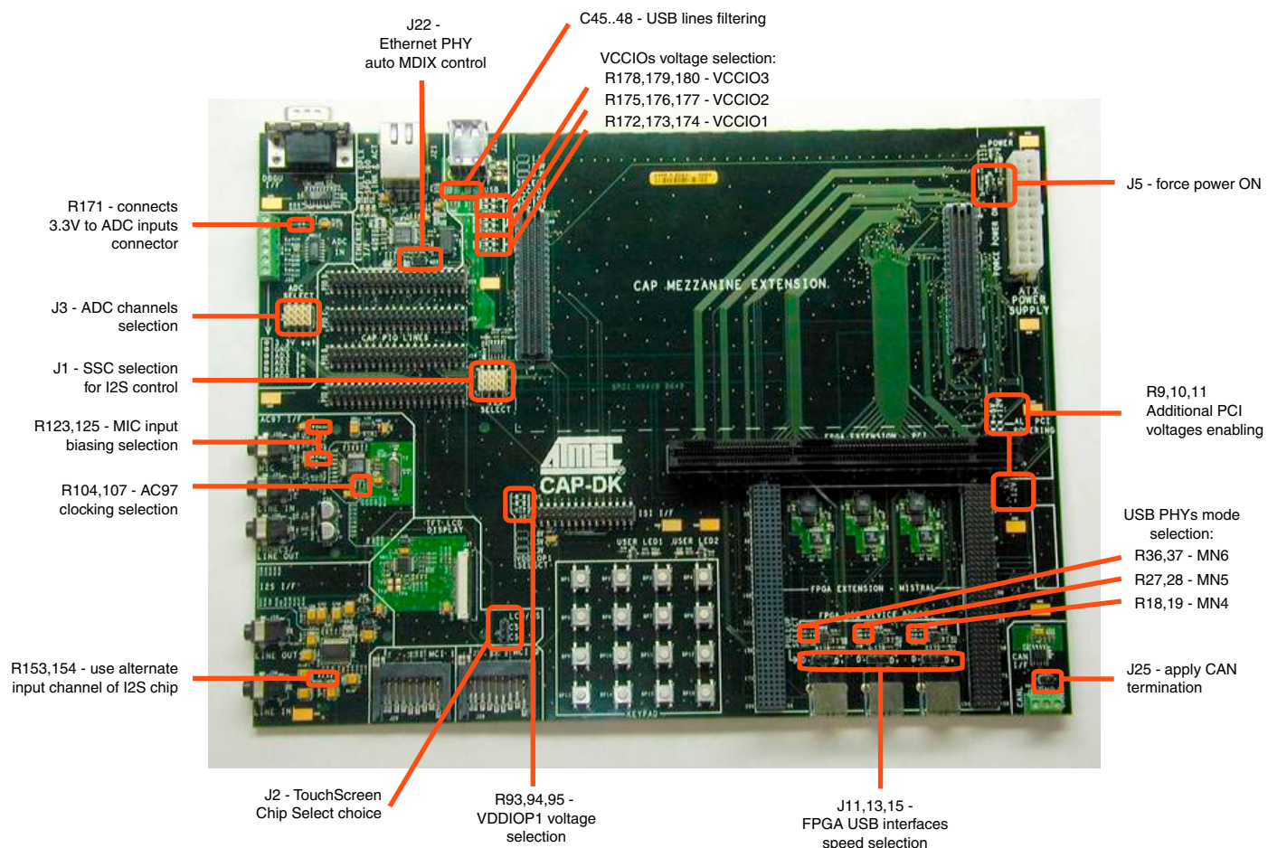
Figure 4-1. AT91CAP-DKM Motherboard
