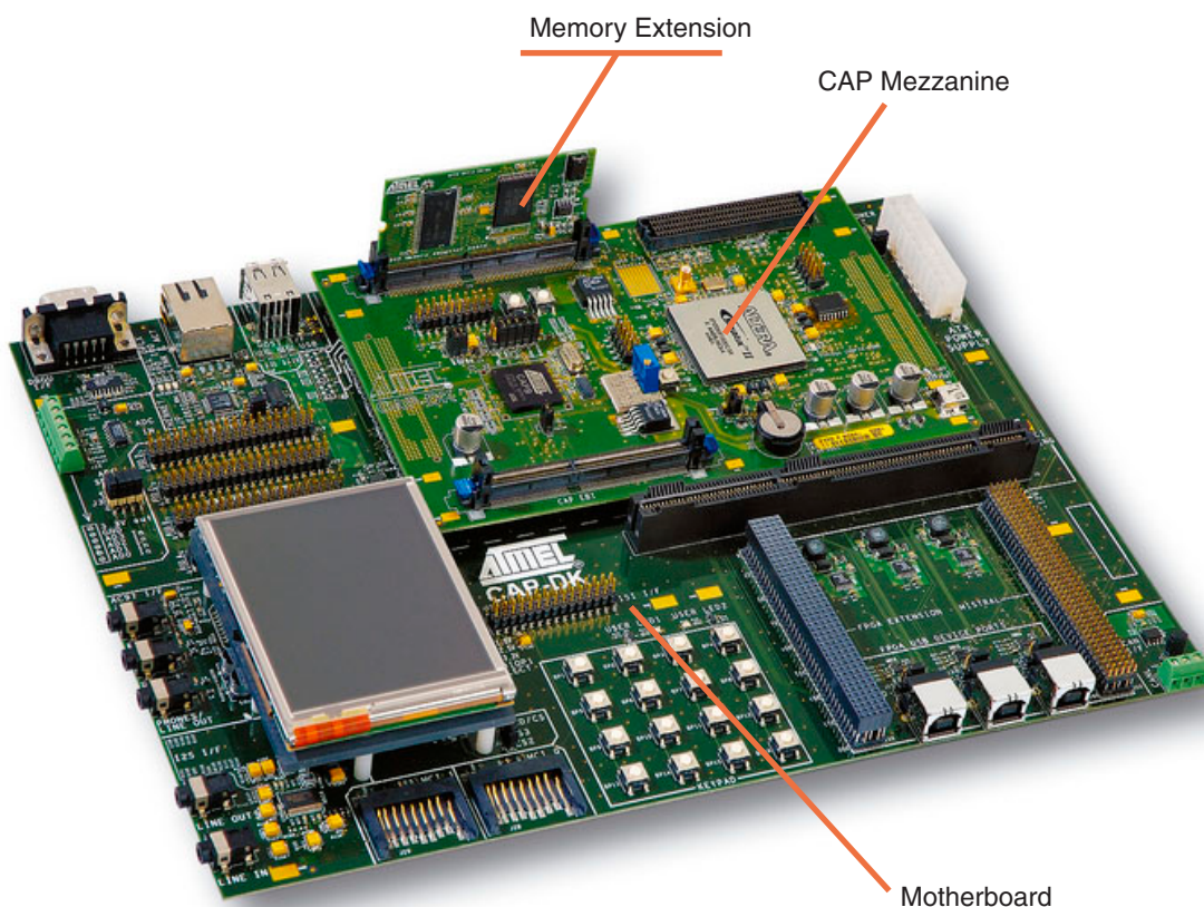
Figure 12-1. AT91CAP-MEM33 Overview
