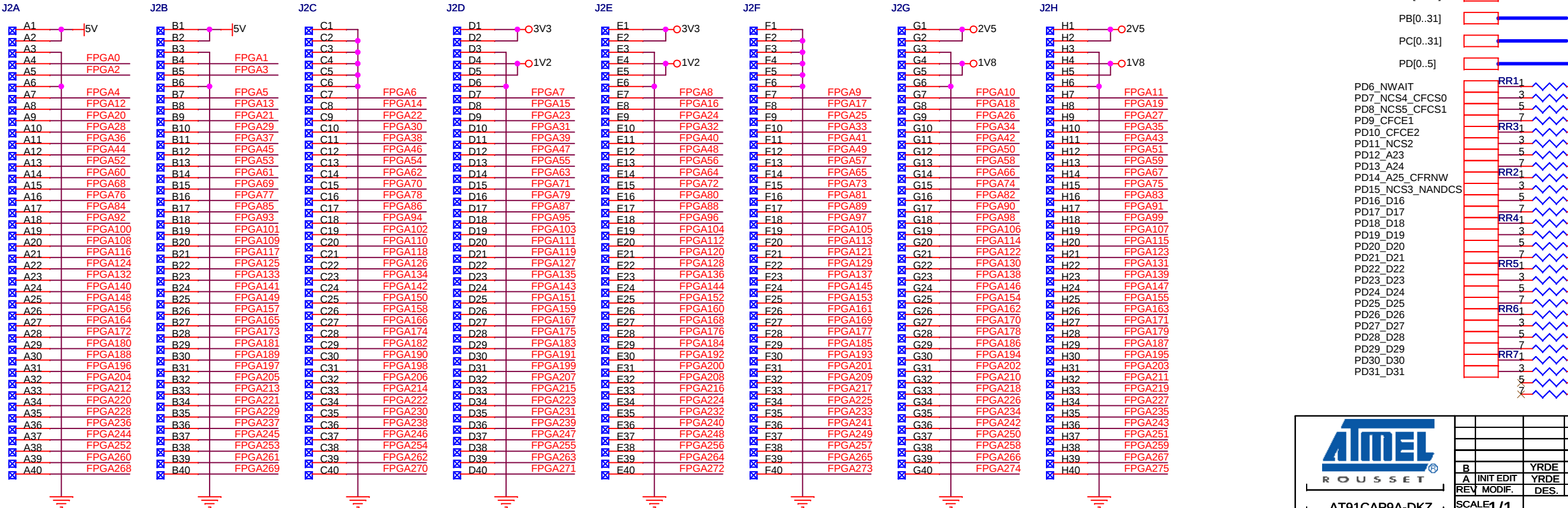
SEAF_40_050_SM_8_2_A_K 320 pins SAMTEC
