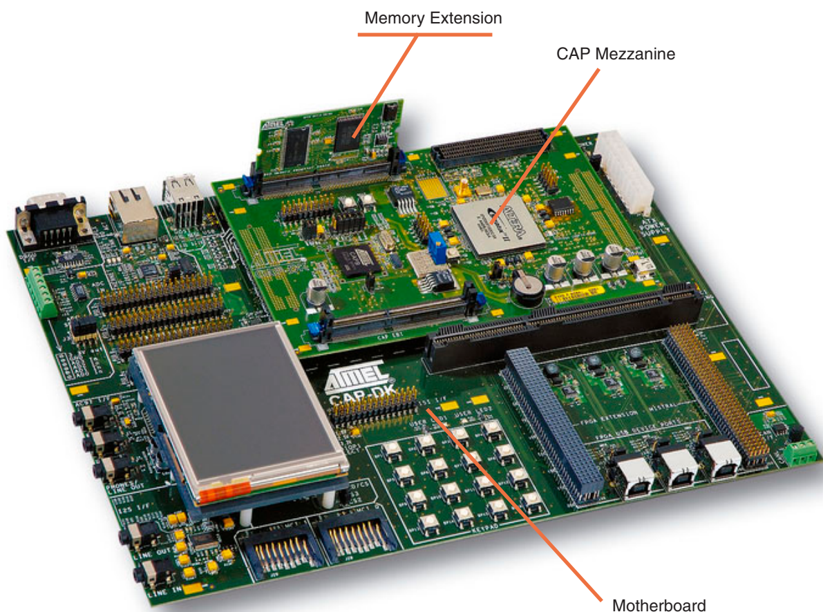
Figure 9-1. AT91CAP-MEM18 Overview
