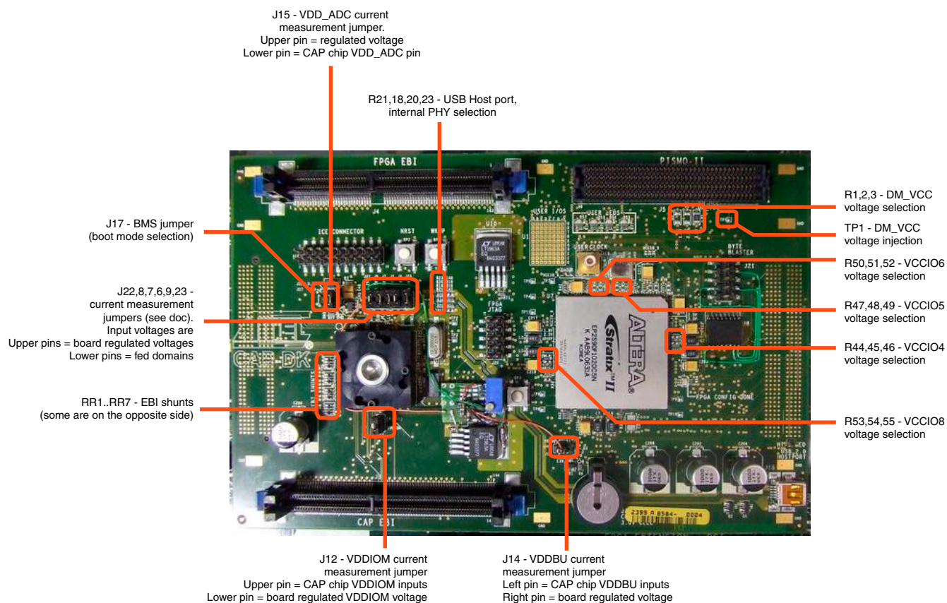
Figure 8-1. AT91CAP9A-DKZ Mezzanine
