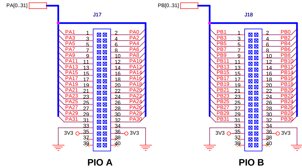
FOUR 40 pins MALE CONNECTORS SAMTEC TSM-120-01-L-DV
