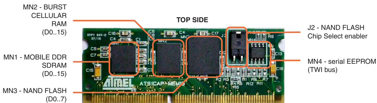
Figure 10-1. AT91CAP-MEM18 Board Layout - Top View
