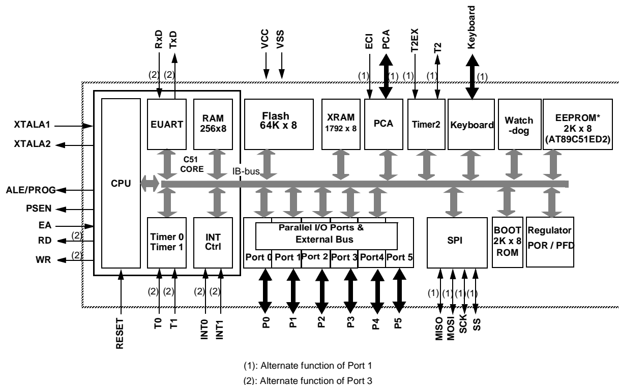
Figure 1. Block Diagram
