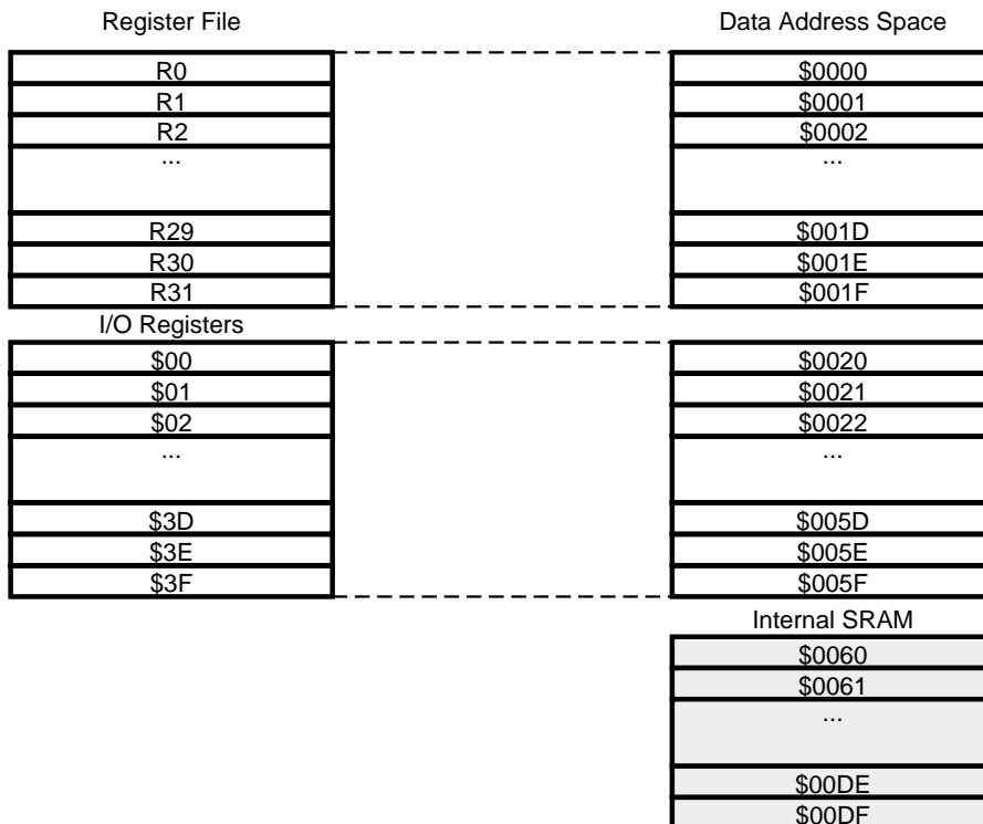
Figure 10. SRAM Organization
