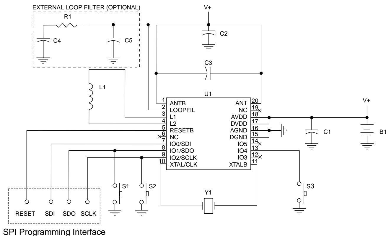
Figure 3. Sample Circuit
