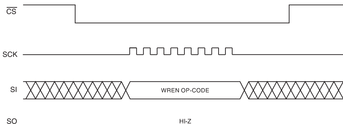
Figure 4. WREN Timing
