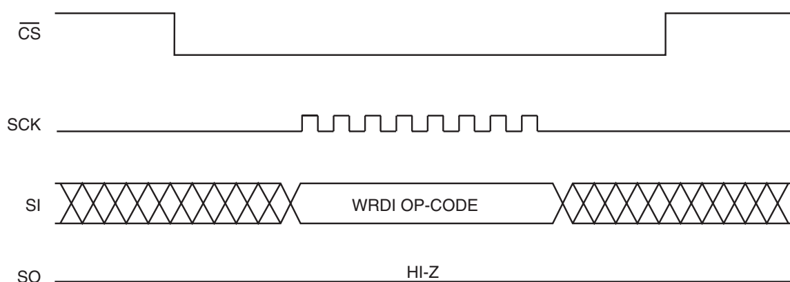
Figure 5. WRDI Timing
