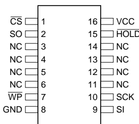
16-lead SOIC
