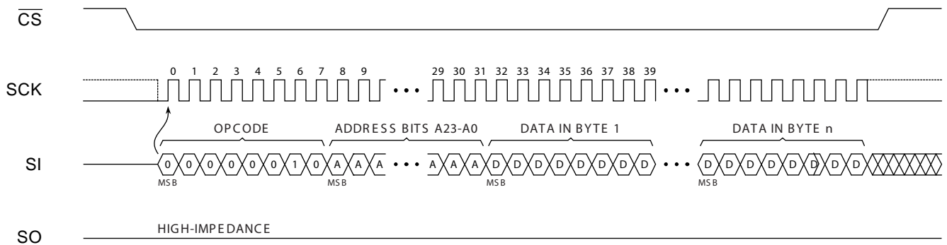
Figure 7-2. Page Program
