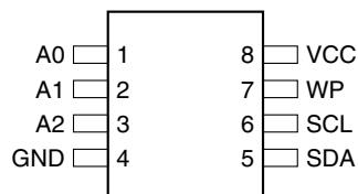
8-lead SOIC
