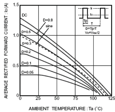
Fig.5 Derating curve ( I_o - T_a )
