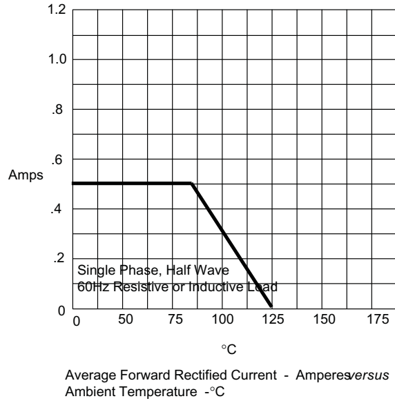
Figure 5 Forward Derating Curve
