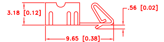
FEMALE CONNECTOR PIN
