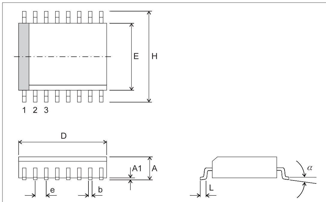
Small Outline Package (SOP) SOP 16 Wide Body (WB)
