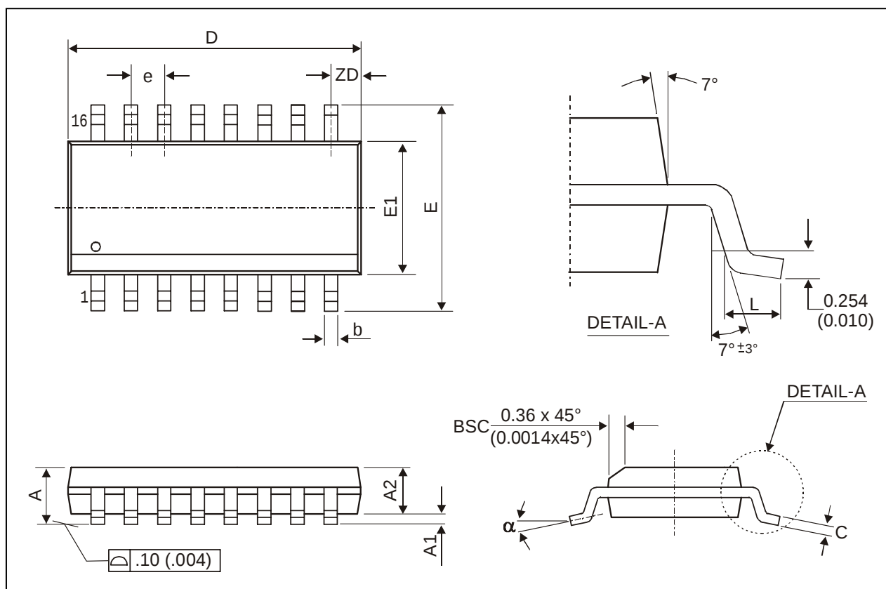
Fig. 8: QSOP16 (Quarter size Small Outline Package)
