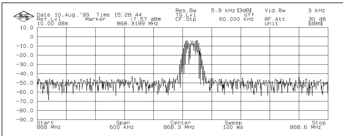
Fig. 7: FM with f_{mod} = 2 kHz, FM input signal with 1 V_{pp} around 1.5 V_{DC} , DATA = HIGH
