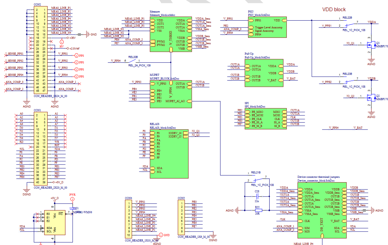
Figure 5: Main schematic
