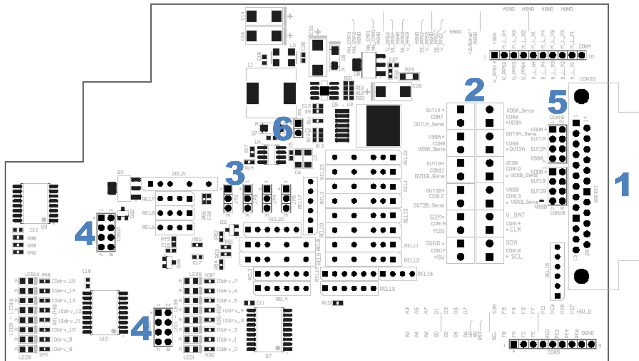
Figure 3: Top layer
