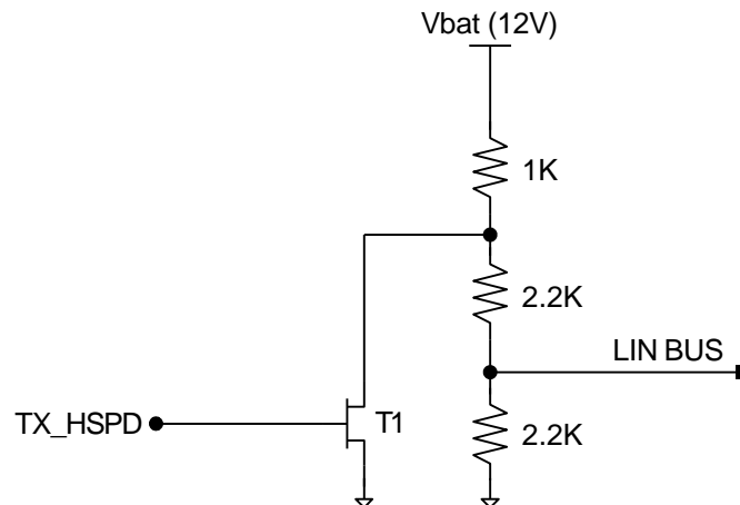
Figure 10: Fast LIN interface
