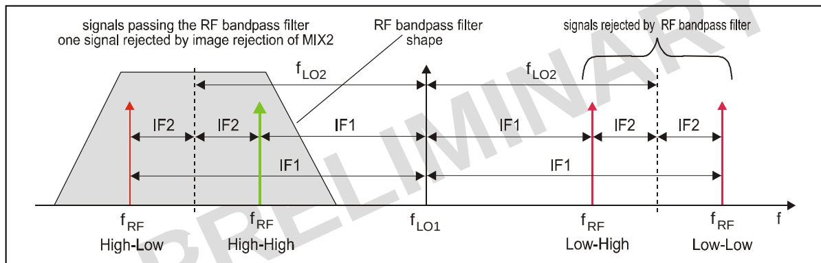
Fig. 2: The four receiving frequencies in a double conversion superheterodyne receiver
