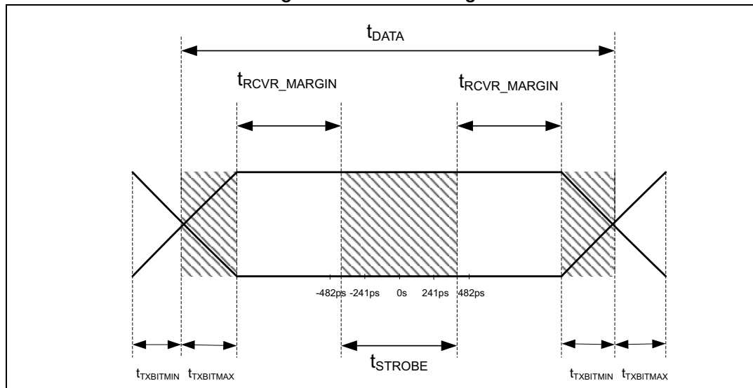
Figure 8. Receiver margins
